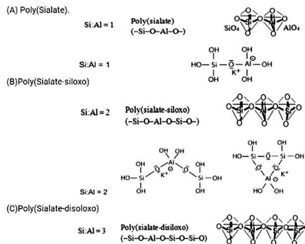
Fig. 2 (A)–(C) Various geopolymer systems based on the \text{Si}:\text{Al} ratio. 8–10
