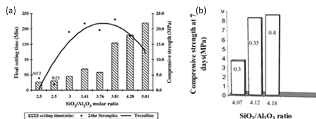
Fig. 23 (a) Compressive strength and final setting time of metakaolin geopolymer with constant H 2 O/Na 2 O molar ratio of 13.6 and varying SiO 2 /Al 2 O 3 ratios. (b) Compressive strength of geopolymer with varying SiO 2 /Al 2 O 3 ratios. 37,120
