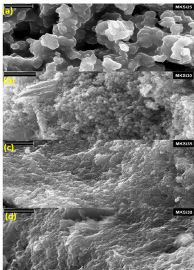
Fig. 31 (a)–(d) High-resolution SEM micrographs of metakaolin with different silica contents (MK = metakaolin, MKSi25– \text{SiO}_2/\text{Al}_2\text{O}_3 = 2.5, MKSi30– \text{SiO}_2/\text{Al}_2\text{O}_3 = 3.0, MKSi35– \text{SiO}_2/\text{Al}_2\text{O}_3 = 3.5, and MKSi38– \text{SiO}_2/\text{Al}_2\text{O}_3 = 3.8). 71
