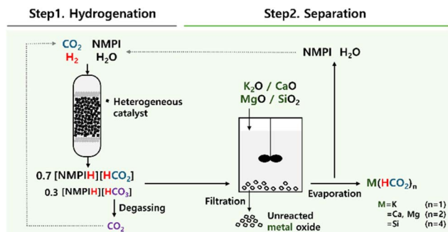
Fig. 3 Schematics of the process for producing metal formate using various metal oxides from \text{CO}_2 hydrogenation adduct made under N -methylpyrrolidine (NMPI)-based basic aqueous solution.
