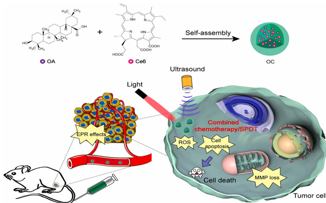
Fig. 7 Schematic of the preparation procedures of self-assembled nanoparticles and their application for synergistic chemo-/sono-photo-dynamic anti-tumor therapy. Copyright © 2021, Elsevier, adapted with permission from ref. 165.
