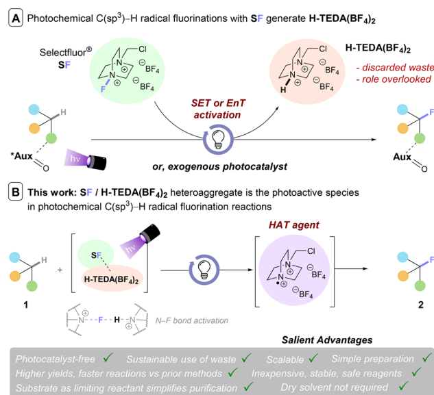
Scheme 1 (A) H-TEDA(BF 4 ) 2 generated after photochemical (radical) C(sp 3 )–H fluorination reactions. (B) This work: SF/H-TEDA(BF 4 ) 2 heteroaggregate as an active species in fluorination reactions.
