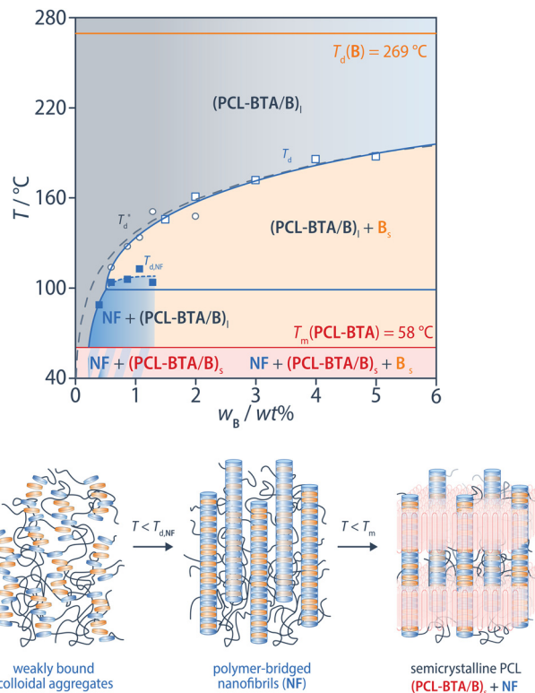
Fig. 8 Phase diagram of PCL-BTA/B blends constructed from T_d^* (open circles), T_{d,NF} (filled squares) and T_d (open squares) obtained from DSC heating scans of PCL-BTA/B blends. (PCL-BTA/B) l – homogeneous melt; NF – nanofibrils; B s – bulk B precipitates; (PCL-BTA/B) s – solid solution. The grey dashed line indicates fitting of the Flory–Huggins model to T_d for PCL/B (see Fig. 2).
