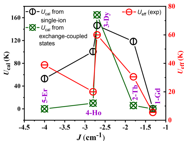
Fig. 8 Comparison of exchange interaction ( J, \text{cm}^{-1} ) with experimental energy barrier ( U_{\text{eff}}, \text{K} ) and computed energy barrier from single-ion as well as exchange-coupled states ( U_{\text{cal}}, \text{K} ) of 1-Gd, 2-Tb, 3-Dy, 4-Ho, and 5-Er .
