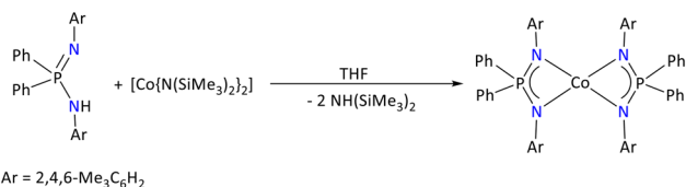
Scheme 32 Synthesis of the homoleptic Co(II) iminophosphonamide complex. 40
