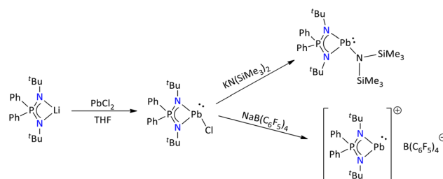
Scheme 20 Iminophosphonamide-stabilized plumbilyumylidene and plumbilyumylidene. 77
