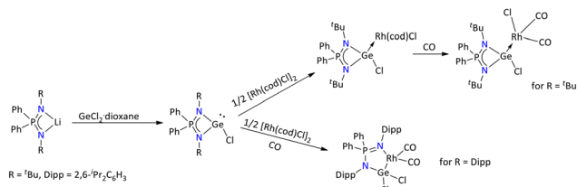
Scheme 18 Syntheses of variably iminophosphonamide-substituted chlorogermylene and their Rh(I) complexes. 78
