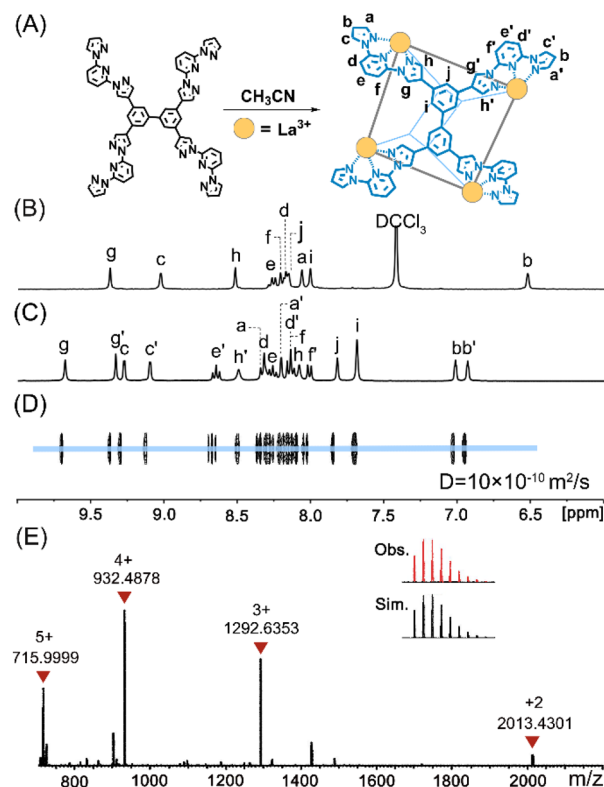
Fig. 1 (A) Self-assembly of L with \text{La}(\text{OTf})_3 . ^1\text{H} NMR spectra (400 MHz, 298 K) of L in \text{CDCl}_3 (B) and \text{La}_4\text{L}_2 in \text{CD}_3\text{CN} (C). (D) DOSY spectra of \text{La}_4\text{L}_2 . (E) ESI-TOF-MS of \text{La}_4\text{L}_2 with the inset showing the observed and simulated isotopic patterns of the +4 peak.
