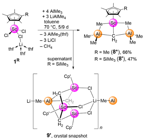
Scheme 3 Synthesis of \text{AlMe}_3 -stabilized methylidenes \text{Cp}^{\text{R}}\text{Sc}(\text{CH}_2)(\text{AlMe}_3)_2 ( 8 R ) via tandem metathesis/thermally induced methyl deprotonation.
