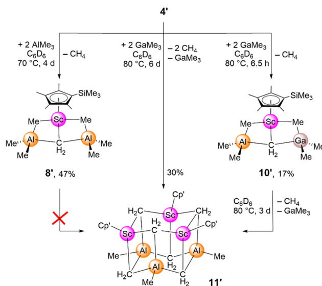
Scheme 5 Reactions of \text{Cp}'\text{Sc}(\text{AlMe}_4)\text{Me} ( 4' ) with \text{AlMe}_3 or \text{GaMe}_3 to form \text{Sc}/\text{Al}_2 methylidene 8' or mixed \text{Sc}/\text{Al}/\text{Ga} methylidene 10' and its reaction to [\text{Cp}'\text{Sc}(\text{CH}_2)_2\text{AlMe}_3] ( 11' ).
