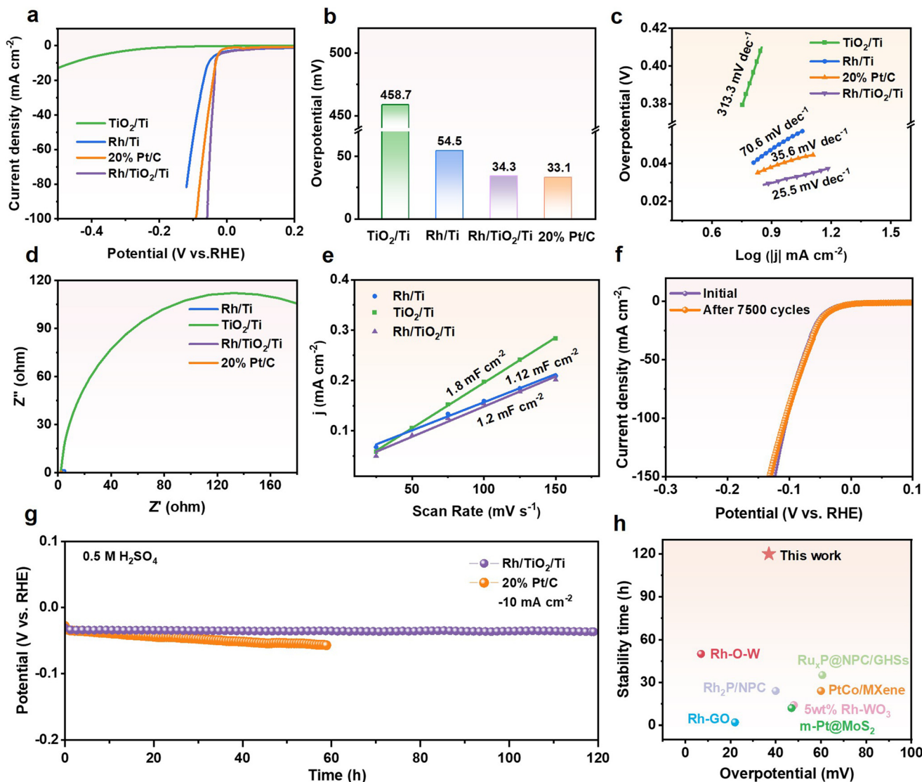
Fig. 5 Electrochemical HER performances in 0.5 M H 2 SO 4 solution. (a) Polarization curves, (b) comparison of overpotentials at -10 \text{ mA cm}^{-2} , and (c) the corresponding Tafel plots of Rh/TiO 2 /Ti, TiO 2 /Ti, Rh/Ti and commercial Pt/C. (d) Nyquist plots of Rh/TiO 2 /Ti, TiO 2 /Ti, Rh/Ti and commercial Pt/C. The enlarged plots are presented in Fig. S12.† (e) Electrochemical double-layer capacitance of Rh/TiO 2 /Ti, TiO 2 /Ti, Rh/Ti. The stability tests for Rh/TiO 2 /Ti. (f) Polarization curves before and after 7500 CV cycles. (g) Comparison of chronopotentiometry curves of Rh/TiO 2 /Ti and commercial Pt/C at -10 \text{ mA cm}^{-2} . (h) Comparison of the overpotential and duration of Rh/TiO 2 /Ti and recently published HER electrocatalysts at -10 \text{ mA cm}^{-2} , with respect to Table S2.†
