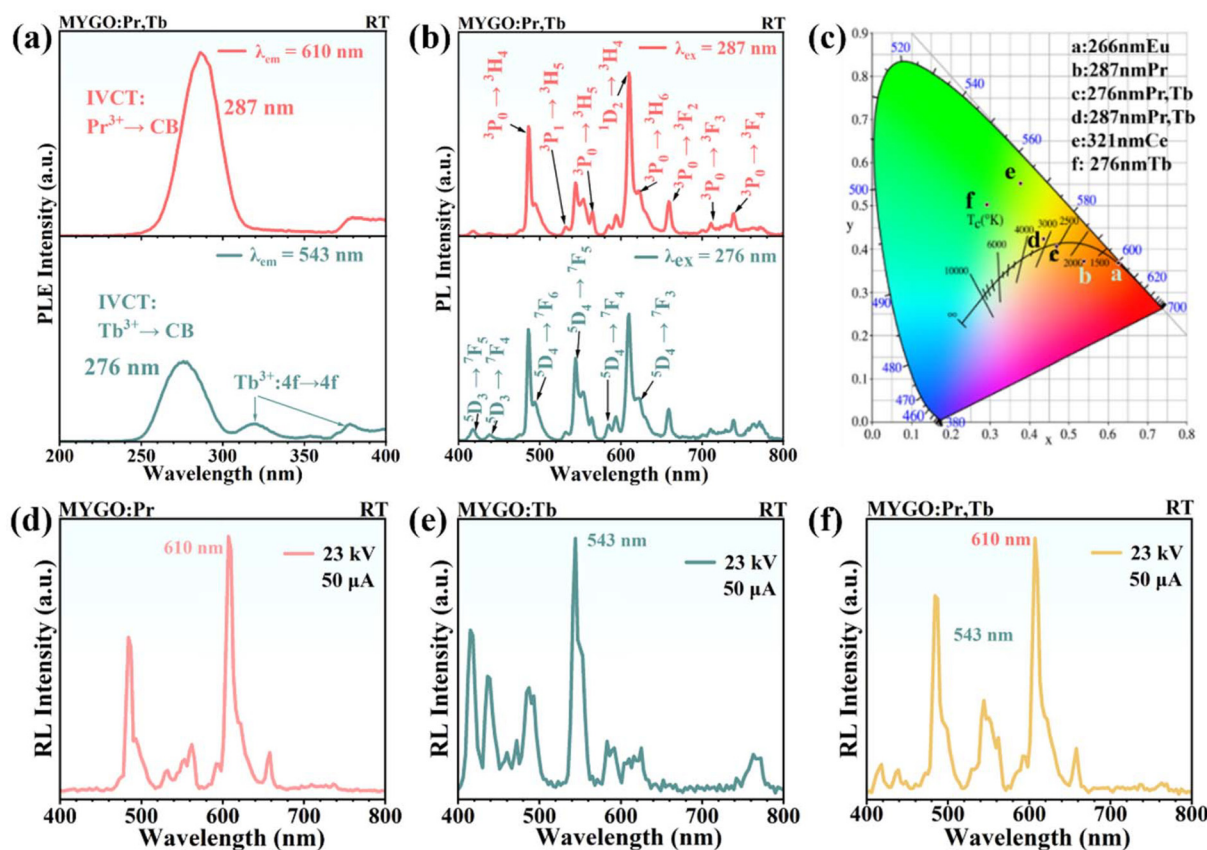
Fig. 3 (a and b) The PLE (a) and PL (b) spectra of the MYGO:Pr,Tb phosphor monitored at 543/610 nm and 276/287 nm, respectively. (c) The Commission International de l'Éclairage (CIE) color coordinates of MYGO:Ln at different wavelengths of UV irradiation. (d–f) The X-ray RL spectra ( U/I = 23 kV, 50 \mu A ) of the samples MYGO:Pr (d), MYGO:Tb (e) and MYGO:Pr,Tb.
