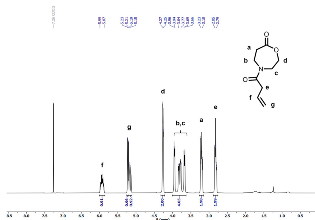
Fig. 2 ^1\text{H} NMR spectrum of 4-(But-3-enoyl)-1,4-oxazepan-7-one (OxP propylene ).
