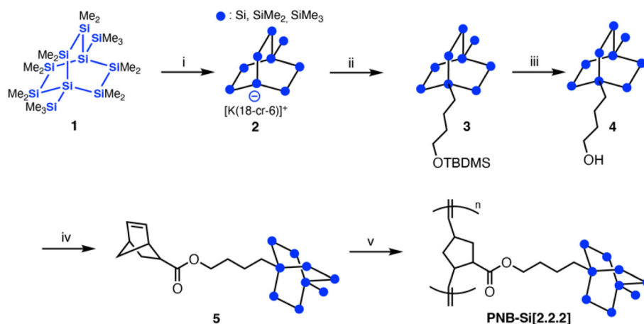
Scheme 1 Synthetic route to monomer 5 and PNB-Si[2.2.2] via ROMP. (i) Potassium tert -butoxide, 18-crown-6, toluene; (ii) 1-bromo-4-( t -butyldimethylsilyloxy)butane, -78\text{ }^{\circ}\text{C} . (iii) acetyl chloride, methanol, tetrahydrofuran, 0\text{ }^{\circ}\text{C} , 40% yield over two steps; (iv) N,N' -dicyclohexylcarbodiimide, 4-dimethylaminopyridine, exo -5-norbornenecarboxylic acid, dichloromethane, 78% yield; (v) Grubbs G2, dichloromethane, room temperature (see Table 1).
