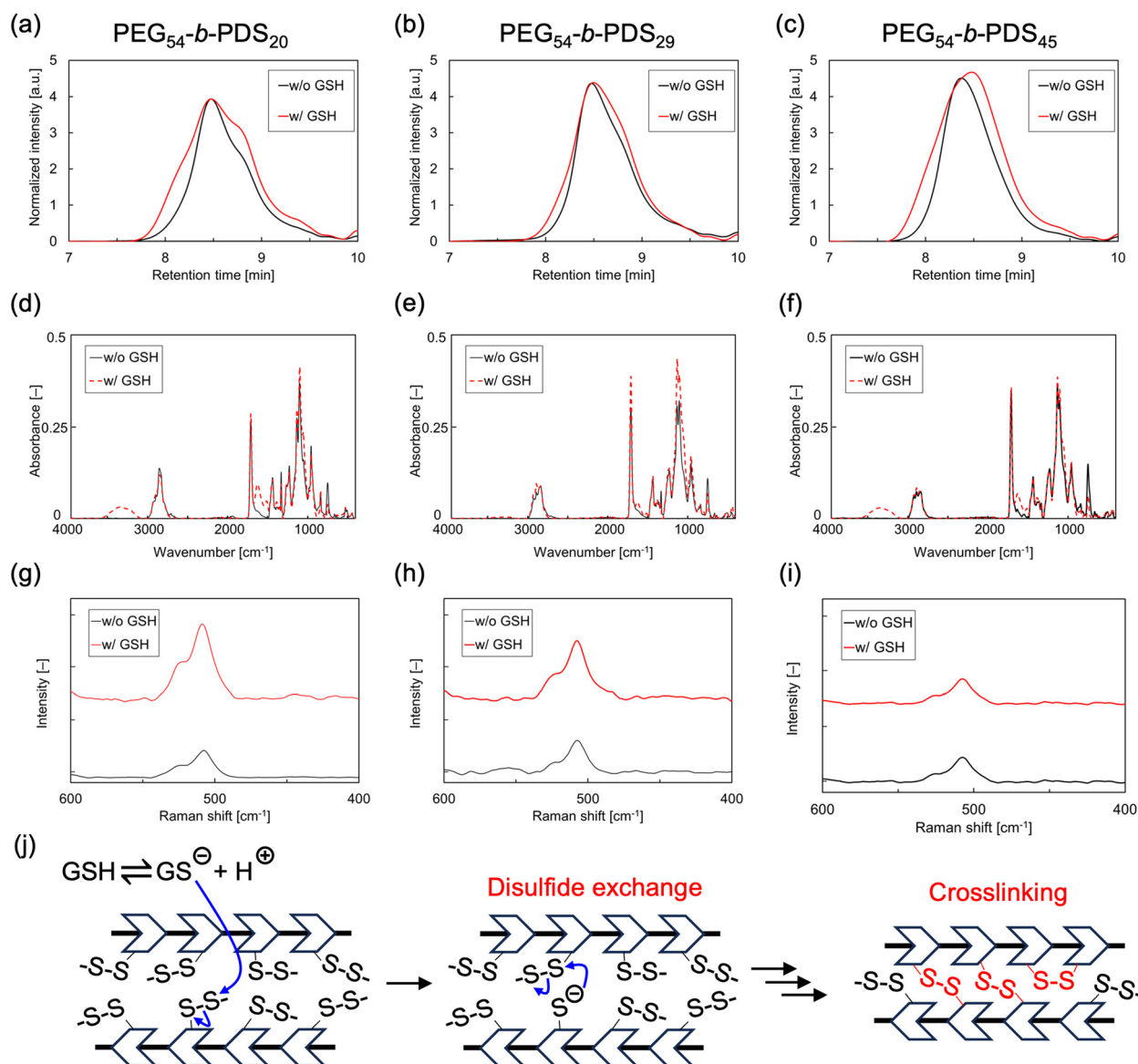
Fig. 3 Analysis of the changes in PEG 54 - b -PDS x ( x = 20, 29 , and 45 ) with the addition of GSH. (a–c) GPC curves of (a) PEG 54 - b -PDS 20 , (b) PEG 54 - b -PDS 29 , and (c) PEG 54 - b -PDS 45 with/without GSH. (d–f) Infrared spectra of (d) PEG 54 - b -PDS 20 , (e) PEG 54 - b -PDS 29 , and (f) PEG 54 - b -PDS 45 with/without GSH. (g–i) Raman spectra of (g) PEG 54 - b -PDS 20 , (h) PEG 54 - b -PDS 29 , and (i) PEG 54 - b -PDS 45 with/without GSH. (j) Estimated molecular conversions of the polymers after the addition of GSH. Thiolate anions of GSH attack the disulfide bonds in the polymer chains to generate new thiolate anions. Subsequently, the generated thiolate anions, which are reactive, attack other disulfide bonds. Chain reactions involving such disulfide exchange reactions result in the overall crosslinking of the polymers.
