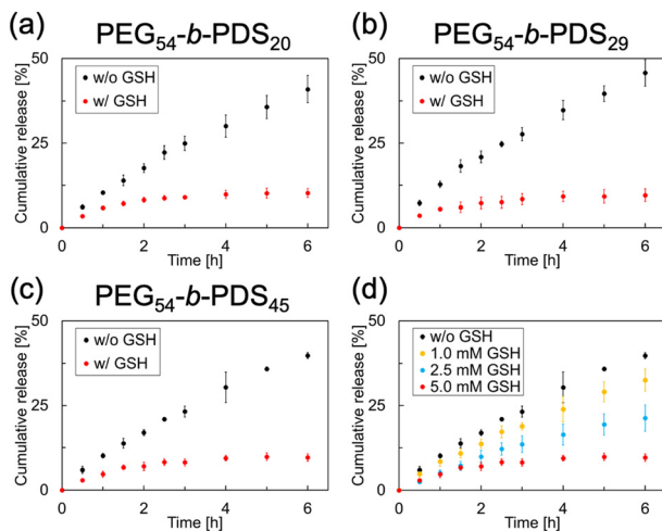
Fig. 6 Release of calcein from polymersomes with/without GSH. (a–c) Cumulative release of calcein from polymersomes comprising (a) PEG 54 -b-PDS 20 , (b) PEG 54 -b-PDS 29 , and (c) PEG 54 -b-PDS 45 with/without GSH (5 mM). (d) GSH-concentration-dependent cumulative release of calcein from polymersomes comprising PEG 54 -b-PDS 45 .
