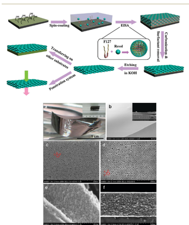
Fig. 4 Top: Schematic preparation process for free-standing mesoporous carbon thin films with a highly ordered Fm\bar{3}m mesostructure by using a coating–etching approach. Bottom: (a) Free-standing OMC film (inset: film transferred onto substrate). (b) SEM images of the free-standing mesoporous carbon films (inset: cross-section). (c)–(e) SEM images from different viewpoints, and (f) cross-section of the free-standing OMC film after carbonization. Reproduced from ref. 25 with permission from ACS, copyright 2025.
