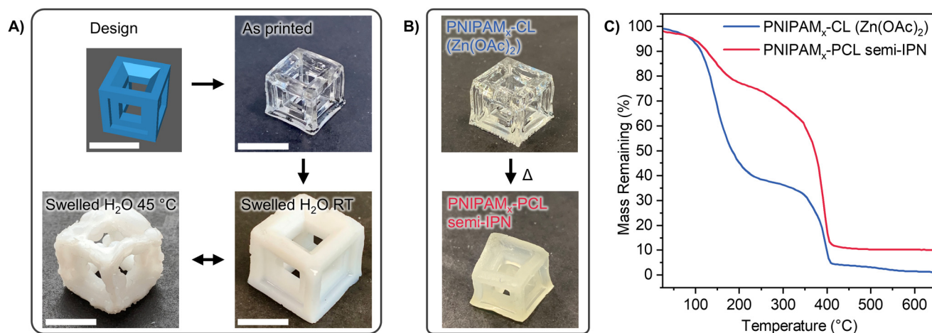
Fig. 7 (A) Images of PNIPAM x -CL 3D printed cube structure showing reversible thermo-responsive swelling in water. Scale bar in all figures represents 1 cm. (B) Images of PNIPAM x -CL (with zinc acetate present) and PNIPAM x -PCL semi-IPN 3D printed materials. (C) TGA thermograms of PNIPAM x -CL with zinc acetate present (blue) and PNIPAM x -PCL semi-IPN (red).
