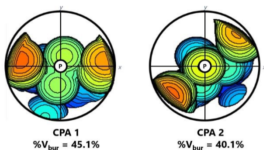
Figure 3 Steric maps based on DFT-optimized CPAs structures viewed down the z -axis. % V_{bur} was determined using a 4.5 Å radius coordination sphere, whose center was displaced by 2.0 Å along the z -axis from the phosphorus atom (The red and the blue zones indicate the more and the less-hindered zones in the catalytic pocket, respectively).
