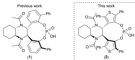
Figure 1 C 2 -symmetric chiral phosphoric acids on a decahydroquinoxaline scaffold
