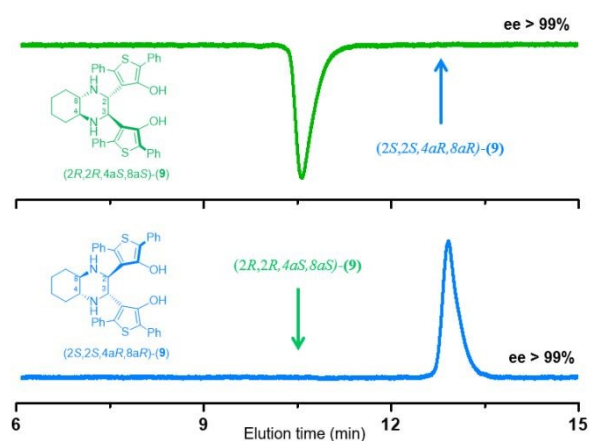
Figure 2. HPLC assessment of the enantiomeric purity of both enantiomers of compound 9 . Chromatographic conditions: column, Chiralpak IB column (250 mm x 4.6 mm); mobile phase, n-hexane/EtOH/DEA (100:10:0.1); temperature, 40 °C; flow rate, 1.0 mL/min; detection, CD at 280 nm.
