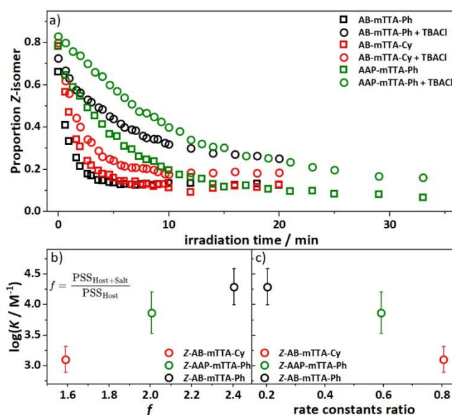
Figure 7. a) Photoisomerization of the Z-isomers of AB-mTTA-Cy, AB-mTTA-(1,3)Ph and AAP-mTTA-(1,3)Ph (1 mM) upon blue (AB, 435 nm) or green (AAP, 520 nm) light irradiation in acetone- d_6 with and without the addition of TBACl (10 equivalents). Plot of K concerning the Z-isomer of the respective host with chloride against b) the fraction f calculated from the PSS with and without salt, and c) the ratio of the photoisomerization rate constants.
