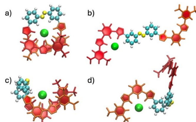
Figure 5. Lowest energy conformers of AB-mTTA-(1,3)Ph bound to chloride calculated by DFT for the E isomer (a), b)) and the Z isomer (c), d))
