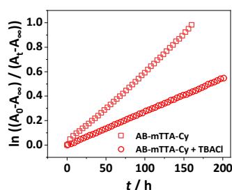
Figure 6. UV-vis spectroscopy study of the build-up of the E-isomer by thermal relaxation of Z-AB-mTTA-Cy (50 \mu M, \text{CHCl}_3 ), monitored by E-isomer absorbance A_E .
