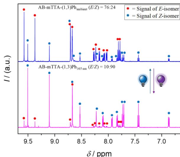
Figure 2. ^1\text{H} -NMR spectra of AB-mTTA-(1,3)Ph (1 mM, acetone- d_6 ) under ambient conditions (top) and after irradiation of 365 nm UV-light (bottom) representing the distinction between signals of the E and Z -isomers, utilized as basis for isomer-specific binding studies by NMR-titrations. For better visibility, only the spectral region of aromatic signals is shown.
