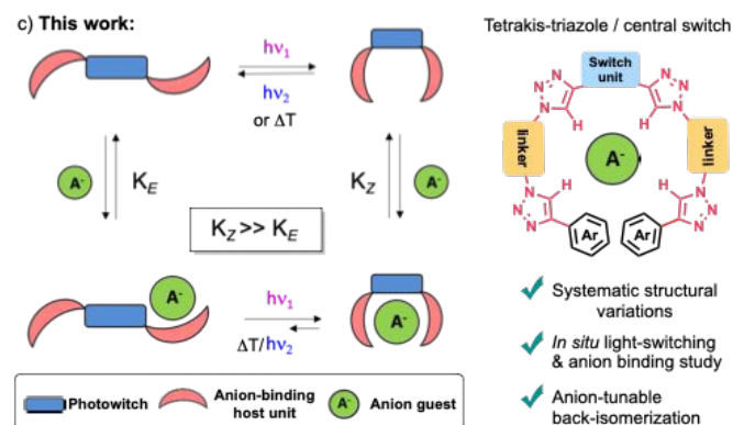
Figure 1. a) Z → E back-isomerization control with azobenzene-urea anion hosts. b) Previously reported azobenzene-triazole photoswitchable anion hosts, and c) concept of tunable photoisomerization towards the underlying anion binding status (left) and our
