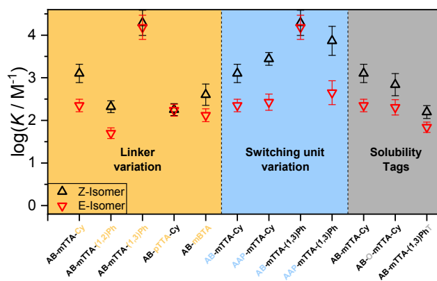
Figure 4: Comparison of the binding constants of different hosts with chloride determined via NMR titration in acetone- d_6 , sorted according to the structure variation.
