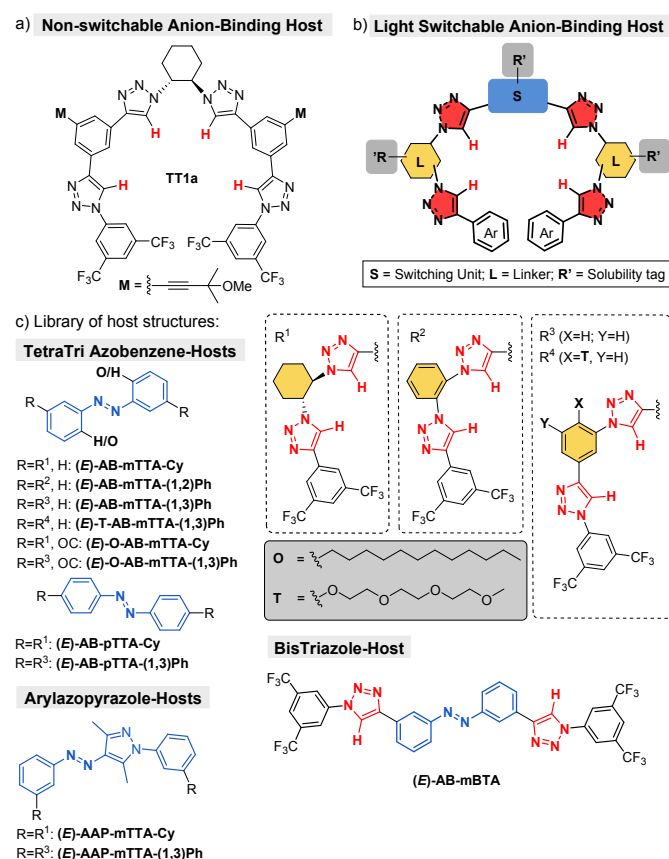
Figure 3. a) Host structure without photoreversibility, TT1a , b) schematic depiction of a photoreversible hosts structure with highlights on the different subunits, c) synthesized hosts with different linkers and substitutions.
