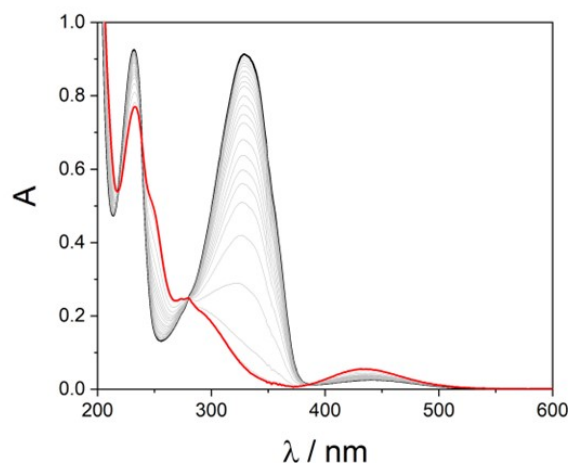
Figure 3. Absorption variations of a 1.6 \times 10^{-5} M solution of EE-4H^+ in CH_3CN (black line) upon irradiation at 365 nm until a photostationary state is reached (red line).
