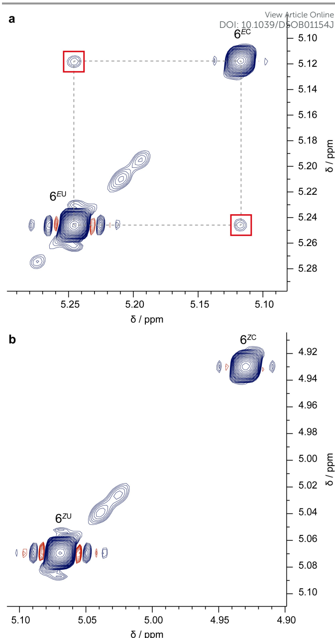
Figure 5. Partial EXSY NMR ( \text{CD}_3\text{CN} , 500 MHz, 298 K, 1.4 mM, t_{\text{mix}} = 600 ms) spectra of (a) an equimolar mixture of EE - 4\text{H}^+ and 2 , and (b) the same sample after exhaustive irradiation at 365 nm. 6^{\text{EU}} and 6^{\text{EC}} in (a) indicates the free and complexed EE -axle, respectively, whereas 6^{\text{ZU}} and 6^{\text{ZC}} in (b) denote the free and complexed ZZ -axle, respectively.
