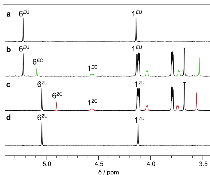
Figure 4. Stacked partial ^1H NMR (500 MHz, CD_3CN , 298 K, 1.4 mM) spectra of (a) axle EE-4H^+ , (b) a 1:1 mixture of EE-4H^+ and crown ether 2 , (c) the same sample after exhaustive irradiation at 365 nm and (d) axle ZZ-4H^+ .
