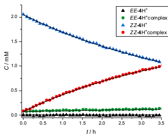
Figure 6. Time-dependent concentration profiles of \text{ZZ-4H}^+\text{C2} (red dots), \text{ZZ-4H}^+ (blue triangles), EE\text{-4H}^+\text{C2} (green dots) and EE\text{-4H}^+ (black triangles). The black lines represent the fitting of the traces. The total concentrations of the axle and the macrocycle, determined from the ^1\text{H} NMR spectra ( \text{CD}_3\text{CN} , 500 MHz, 298 K) are 2.2 mM and 24 mM, respectively.
