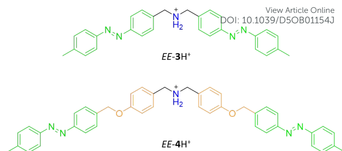
Figure 2. Structure formula of the symmetric axes EE-3H^+ and EE-4H^+ .
