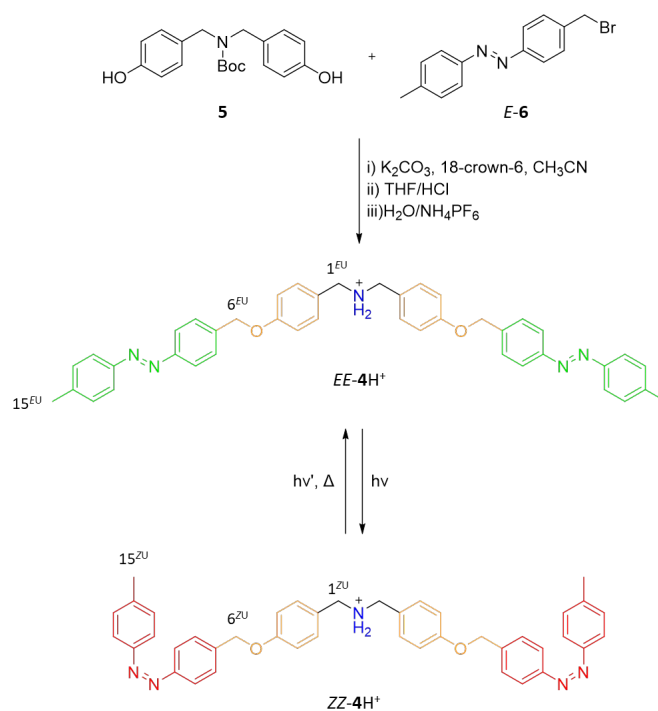
Scheme 1. Convergent synthetic pathway to EE-4H^+ and photoisomerization product ZZ-4H^+ .
