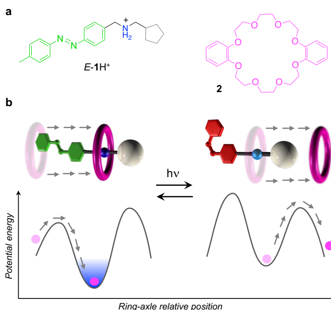
Figure 1. (a) The molecular components of a pseudorotaxane-based photochemically driven molecular pump. (b) Cartoon representation of the photoinduced directional threading-unthreading movement and simplified potential energy diagram showing the light-dependent modulation of maxima and minima (ratcheting) at the basis of the pump mechanism.
