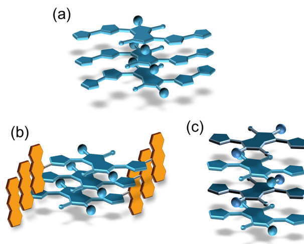
Fig. 7 Pictorial representation of the aggregation modes observed for three different classes of DPP dyes recently investigated by our group: (a) \text{Th}_2 -DPP- \text{Th}_2 derivatives, (b) Anth-Th-DPP-Th-Anth derivatives, (c) Th-DPP-Th derivatives.
