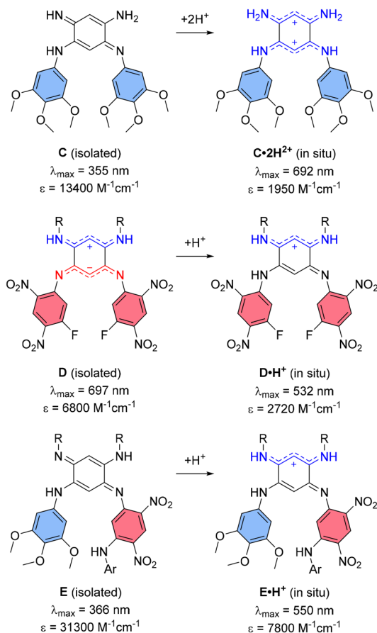
Fig. 2 Previous works on diaminobenzoquinone diimines (R = \text{C}_6\text{H}_{17} ; Ar = \text{C}_6\text{H}_2(\text{OCH}_3)_3 ) with their absorption maxima and corresponding molar extinction coefficients in solution (in methanol–water for C , in DCM for D and E ).
