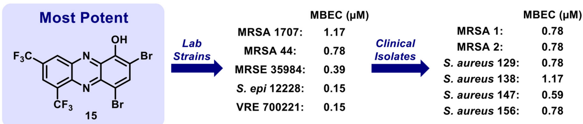
Fig. 4 (A) Select halogenated phenazine biofilm eradication activities. (B) Representative MBEC images of halogenated phenazines evaluated in Calgary Biofilm Device (CBD) assays. (C) Biofilm eradication profile for HP 15. Note: *Compounds were tested from 0.2 \mu\text{M} to 200 \mu\text{M} (10 mM DMSO stock solution). **Compounds were tested from 0.1 \mu\text{M} to 100 \mu\text{M} (5 mM DMSO stock solution). ***Compounds were tested from 2 \mu\text{M} to 2000 \mu\text{M} (100 mM DMSO stock solution).
