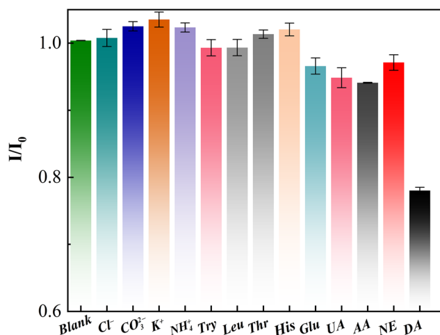
Fig. 7 Selectivity of the DA detection. I_0 represents the initial intensity and I represents the intensity with interfering species. Reaction conditions: the concentration of all the metal ions is 0.2 mM, the concentration of all the amino acids and glucose are 0.5 \mu\text{M} , and the concentrations of DA, NE, AA, and UA are 0.5 \mu\text{M} , 50 \mu\text{M} luminol in PBS (pH 11.0), 2000 \mu\text{M} H 2 O 2 , and 50 \mu\text{g mL}^{-1} Mn-MOFs.
