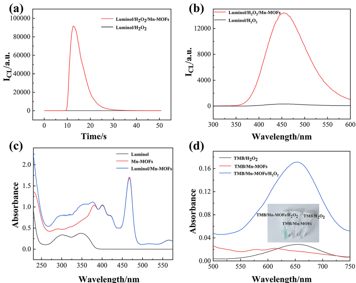
Fig. 3 (a) CL intensity–time curves and (b) CL spectra of the luminol/ \text{H}_2\text{O}_2 system in the absence (black line) and presence (red line) of Mn-MOFs. Reaction conditions: 50 \mu\text{M} luminol in PBS (pH 11.0), 2000 \mu\text{M} \text{H}_2\text{O}_2 , and 50 \mu\text{g mL}^{-1} Mn-MOFs. (c) UV-vis absorption spectra of luminol (black line), Mn-MOFs (red line), and luminol/Mn-MOFs (blue line). (d) UV-vis absorption spectra of TMB/ \text{H}_2\text{O}_2 (black line), TMB/Mn-MOFs (red line), and TMB/Mn-MOFs/ \text{H}_2\text{O}_2 (blue line) in a 0.2 \text{ M} HAC/NaAc buffer solution (pH 4.0). Inset: images captured after 2 hours (left to right): TMB/Mn-MOFs/ \text{H}_2\text{O}_2 , TMB/Mn-MOFs, and TMB/ \text{H}_2\text{O}_2 . Reaction conditions: 1 \text{ mM} TMB, 100 \text{ mM} \text{H}_2\text{O}_2 , and 10 \mu\text{g mL}^{-1} Mn-MOFs.
