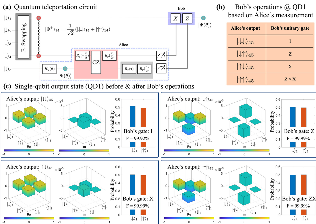
Fig. 5 Quantum teleportation module: (a) a quantum teleportation module implemented with our five quantum dot (QD) system is shown in a logical level. Once the entanglement swapping process (Fig. 4(a)) is completed, its output state is utilized as a quantum channel to teleport an arbitrary single-qubit state that is prepared by the sender (Alice) with a Y -rotation ( R_Y(\theta) ) of the spin in QD5. This single-qubit state, together with the spin of QD4, is then subjected to a Bell measurement. (b) Depending on the outcome of the Bell measurement, the receiver (Bob) conducts a pre-defined set of logic operations to the spin of QD1 to get the final outcome. (c) Density matrices of the spin state in QD1 prior to Bob's single-qubit operations are presented. Bar graphs show the spin probabilities of QD1 that are obtained after conduction of Bob's logic operations.
