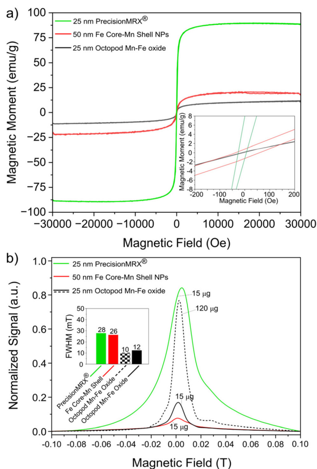
Fig. 3 (a) The field-dependent magnetization curves and (b) the corresponding normalized PSD for 25 nm octopod-shaped Mn-Fe oxide NPs, 50 nm Fe core-Mn shell NPs, and 25 nm commercial PrecisionMRX® iron oxide NPs. Relaxometry measurements were conducted at a sample concentration of 15 \mu\text{g} of total Fe and Mn per 1 mL solvent, except for the hatched graph, which represents signal data for 25 nm octopod Mn-Fe oxide NPs at a concentration of 120 \mu\text{g} of total Fe and Mn per 1 mL solvent.
