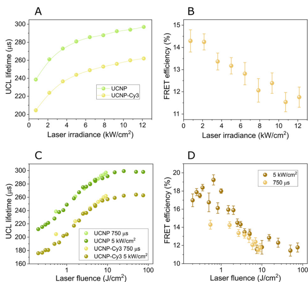
Fig. 3 (A) UCL luminescence lifetime as a function of laser irradiance for CS1 core-shell nanoparticles (with active shell 5.5 nm) with and without dye for a fixed pulse width of 750 \mu\text{s} . Error bars are included but not visible as they are smaller than the symbol size. (B) FRET efficiency obtained from data shown in A. (C) UCL lifetime extracted from Fig. 2C (dark-colored symbols) and A (light-colored symbols) as a function of laser fluence, measured by varying the laser pulse width and laser power, respectively. (D) FRET efficiency calculated from the UCL lifetime data shown in C.
