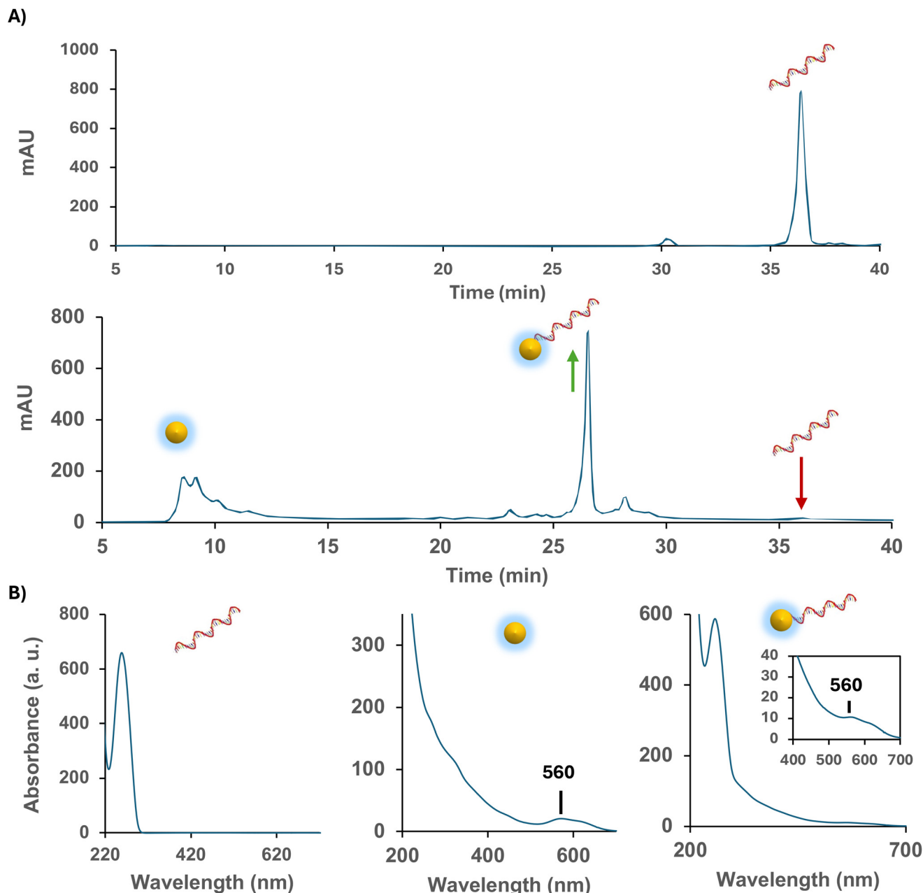
Fig. 3 (A) Top shows the RP-HPLC analysis for thiol-17mer, while the bottom shows the RP-HPLC analysis for Au 18 (SG) 14 conjugated with thiol-17mer with a linear gradient from 0% to 12% of acetonitrile in 10 mM TEAA, and detection at 260 nm. (B) Corresponding absorbance measurements of the three peaks assigned to thiol-17mer, Au 18 (SG) 14 , and Au 18 (SG) 13 -17mer (1) .
