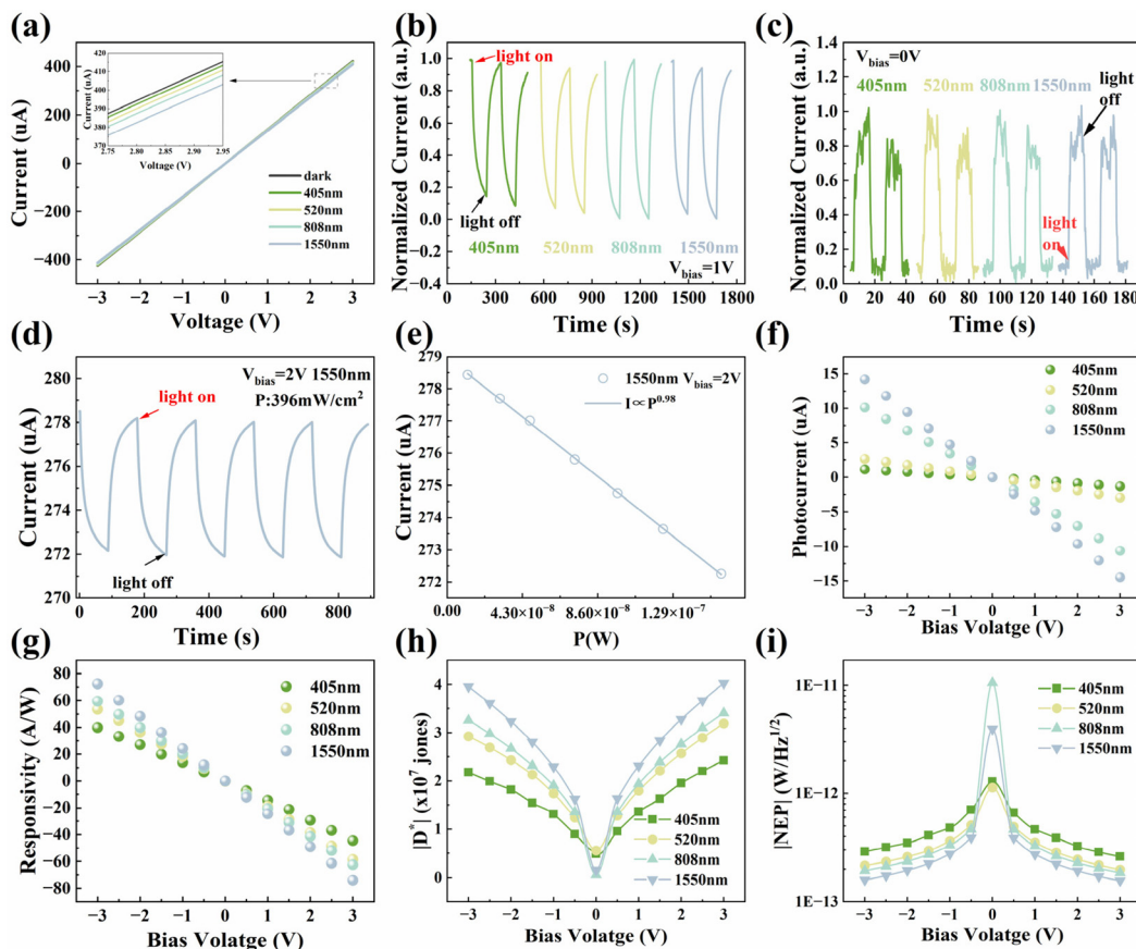
Fig. 2 Photoelectric properties of \text{Bi}_2\text{Se}_3\text{-PtSe}_2 heterojunction photodetectors at UV to IR wavelengths. (a) I - V characteristic curves of the device under different-wavelength irradiation and in the dark state. Optical response of the device under 405–1550 nm wavelength irradiation at (b) V_{\text{bias}} = 1 V and (c) V_{\text{bias}} = 0 V. Stability curves of the photocurrent of the device under 1550 nm illumination (d) and the fitted curves of the current versus the power intensity (e), V_{\text{bias}} = 2 V. Photocurrent (f), responsivity (g), specific detectivity (h), and noise-equivalent power (i) versus bias voltage for devices irradiated at 405–1550 nm.
