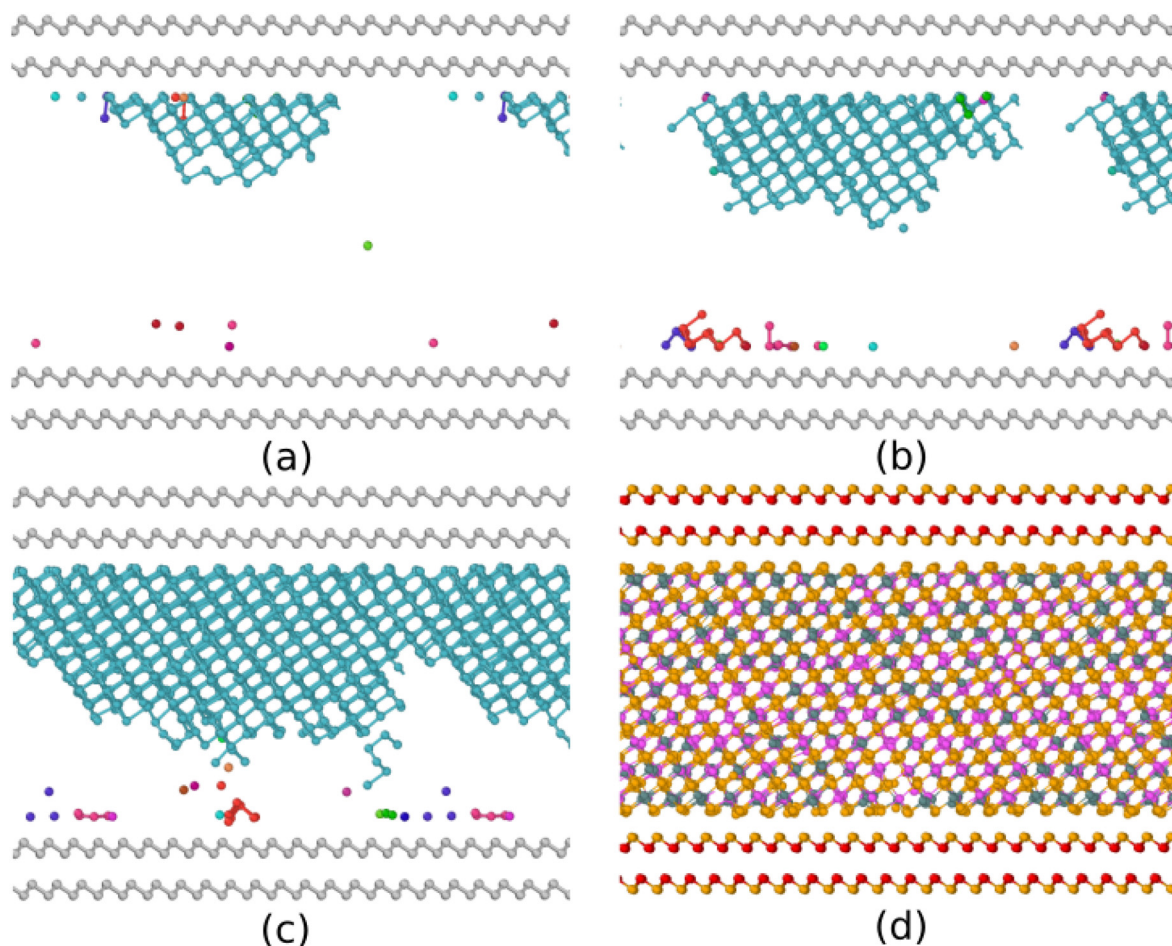
Fig. 8 Simulation of the crystallization of a 3528-atom slab of amorphous GST capped by bilayers mimicking confinement by TiTe 2 in GST/TiTe 2 superlattices at a lower density of the GST slab (SL-LD', see text). Snapshots at different times at 750 K are shown for (a) 0.5 ns, (b) 0.75 ns, and (c) 1 ns. Crystallization starts at the surfaces of the amorphous slab, albeit the capping layers do not act as nucleation centers. Only crystalline atoms, identified by the Q_4^{\text{ot}} order parameter (see Section 2), are shown. Different crystalline nuclei have different colors. (d) Final configuration after 1.2 ns. The color code is the same as Fig. 1.
