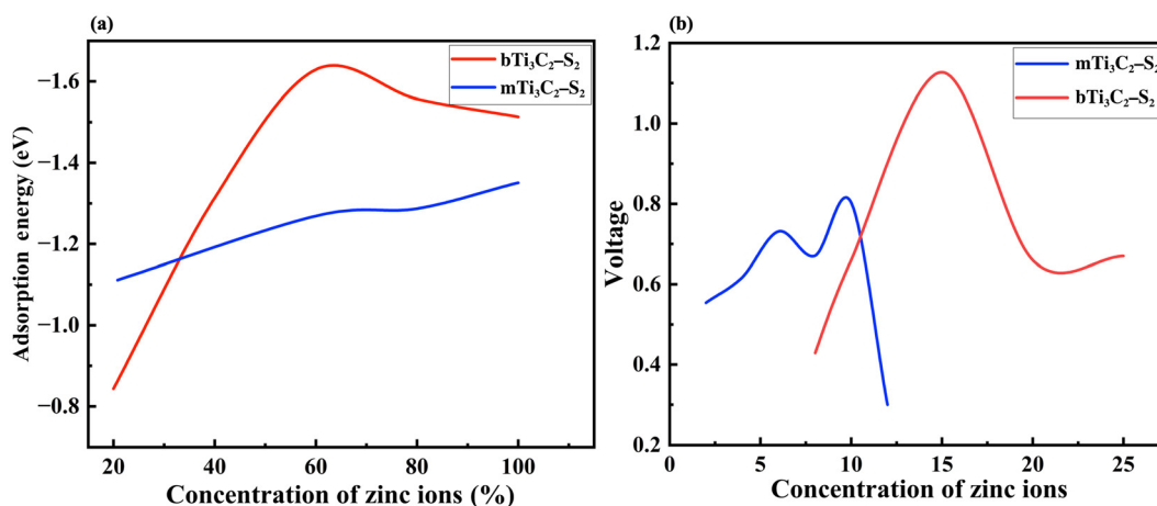
Fig. 3 Representations of (a) the adsorption energy versus Zn-ion concentration curve, showing the variation in adsorption energy with Zn-ion concentration for m Ti 3 C 2 -S 2 and b Ti 3 C 2 -S 2 MXene structures and (b) the voltage profile of m Ti 3 C 2 -S 2 and b Ti 3 C 2 -S 2 MXene structures with respect to Zn-ion concentration.
