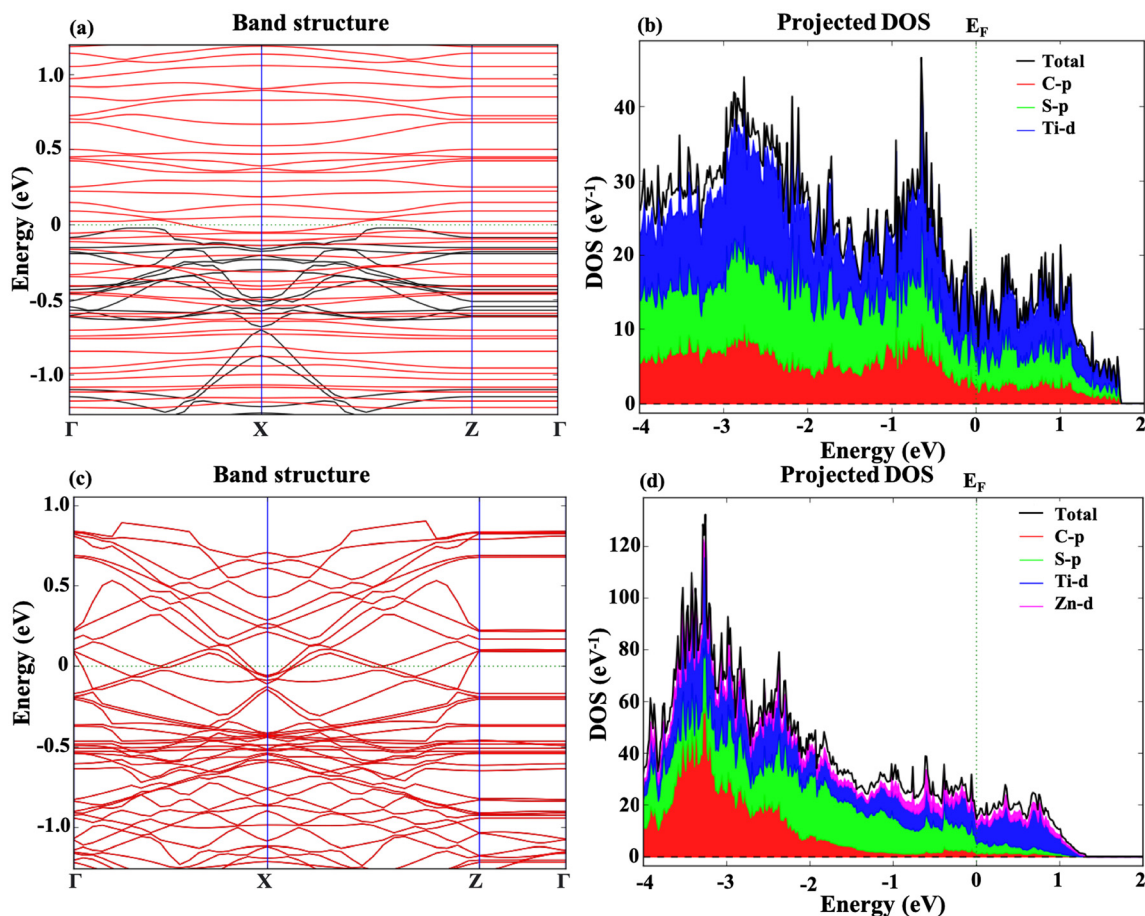
Fig. 5 Representations of (a) the band structure of the b \text{Ti}_3\text{C}_2\text{-S}_2 MXene before Zn-ion intercalation; (b) PDOS of the b \text{Ti}_3\text{C}_2\text{-S}_2 MXene before Zn-ion intercalation; (c) band structure of the b \text{Ti}_3\text{C}_2\text{-S}_2 MXene after Zn-ion intercalation; and (d) PDOS of the b \text{Ti}_3\text{C}_2\text{-S}_2 MXene after Zn-ion intercalation.
