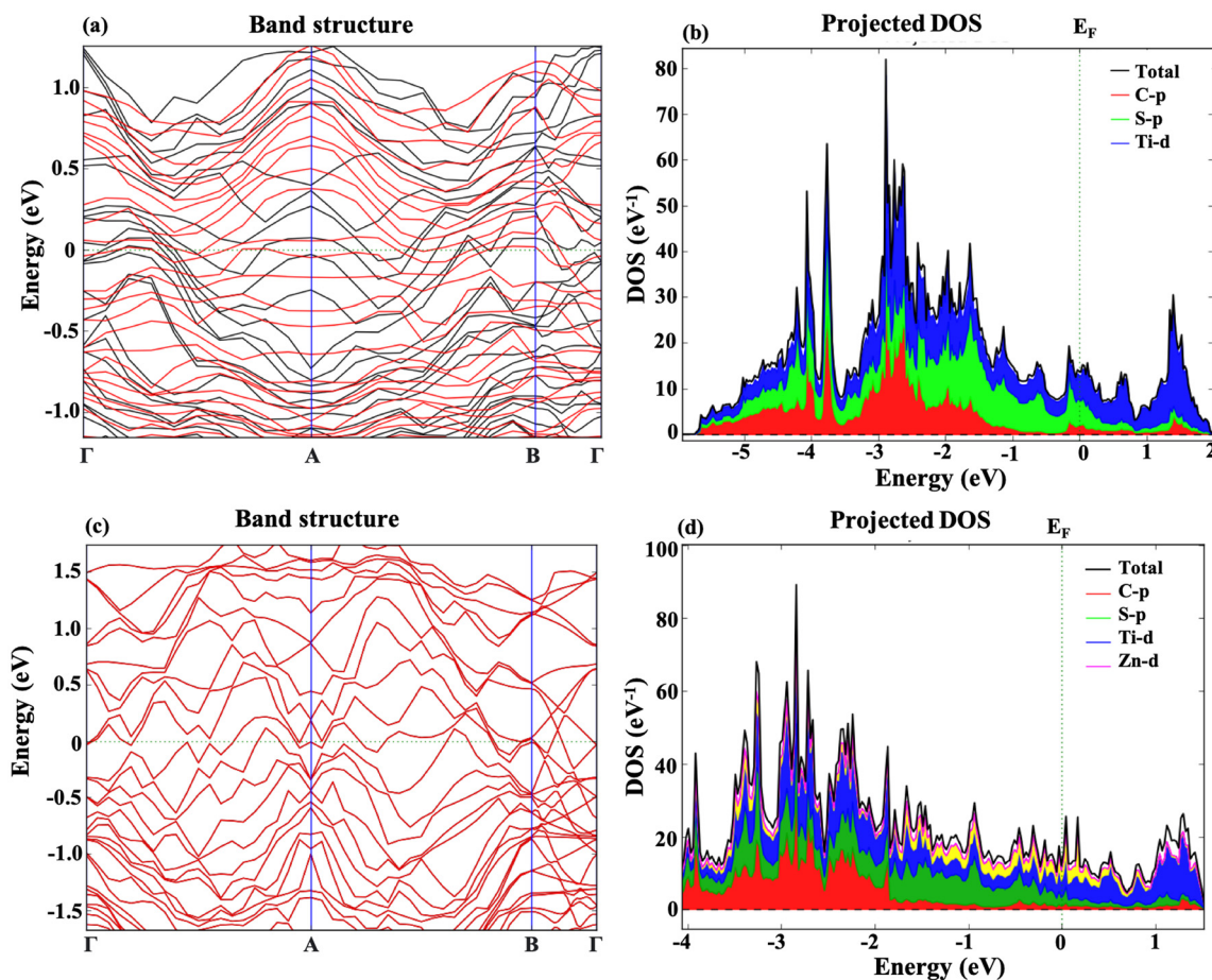
Fig. 4 Representations of (a) the band structure of the m Ti 3 C 2 S 2 MXene before Zn-ion adsorption; (b) PDOS of the m Ti 3 C 2 S 2 MXene before Zn-ion adsorption; (c) the band structure of the m Ti 3 C 2 S 2 MXene after Zn-ion adsorption; and (d) PDOS of the m Ti 3 C 2 S 2 MXene after Zn-ion adsorption.
