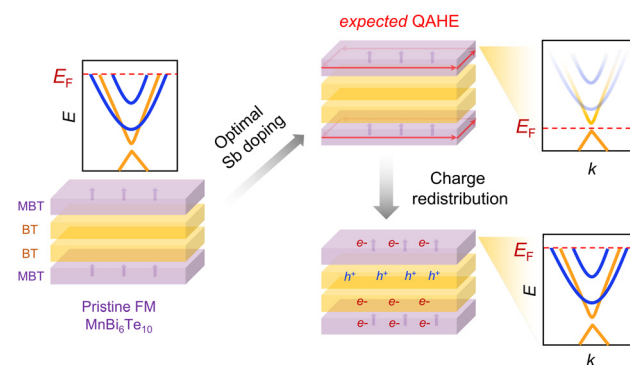
Fig. 4 Charge redistribution in the charge neutral Mn(Bi 0.82 Sb 0.18 ) 6 Te 10 prevents the material from realizing the quantum anomalous Hall effect. Instead of the homogenous charge neutrality, the imbalance of the charge distribution always leaves the MBT layer electron-doped.
