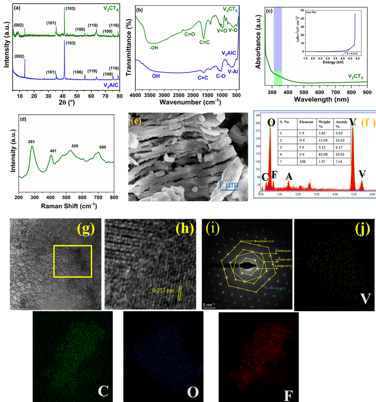
Fig. 1 (a) XRD pattern measured within the range of 2\theta = 5^\circ\text{--}80^\circ , (b) FTIR spectra captured within the range of 4000\text{--}500\text{ cm}^{-1} , (c) UV-Vis absorption spectrum of \text{V}_2\text{CT}_x across the range of 250\text{--}900\text{ nm} . Inset: Tauc plot estimating the optical band gap, (d) Raman spectra of \text{V}_2\text{CT}_x , (e) SEM Image and (f) EDX spectra of the as-synthesized \text{V}_2\text{CT}_x , (g) TEM image of the \text{V}_2\text{CT}_x MXene, (h) HRTEM image, (i) SAED pattern and (j) EDX-mapping analysis of the \text{V}_2\text{CT}_x MXene.
