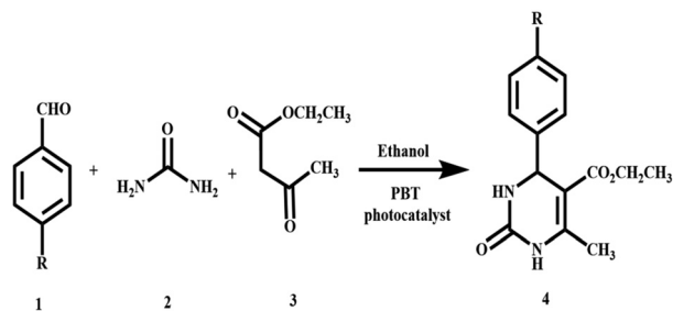
Fig. 1 Reaction conditions for green synthesis of DHPs with catalysis by the PBT photocatalyst under solar light.
