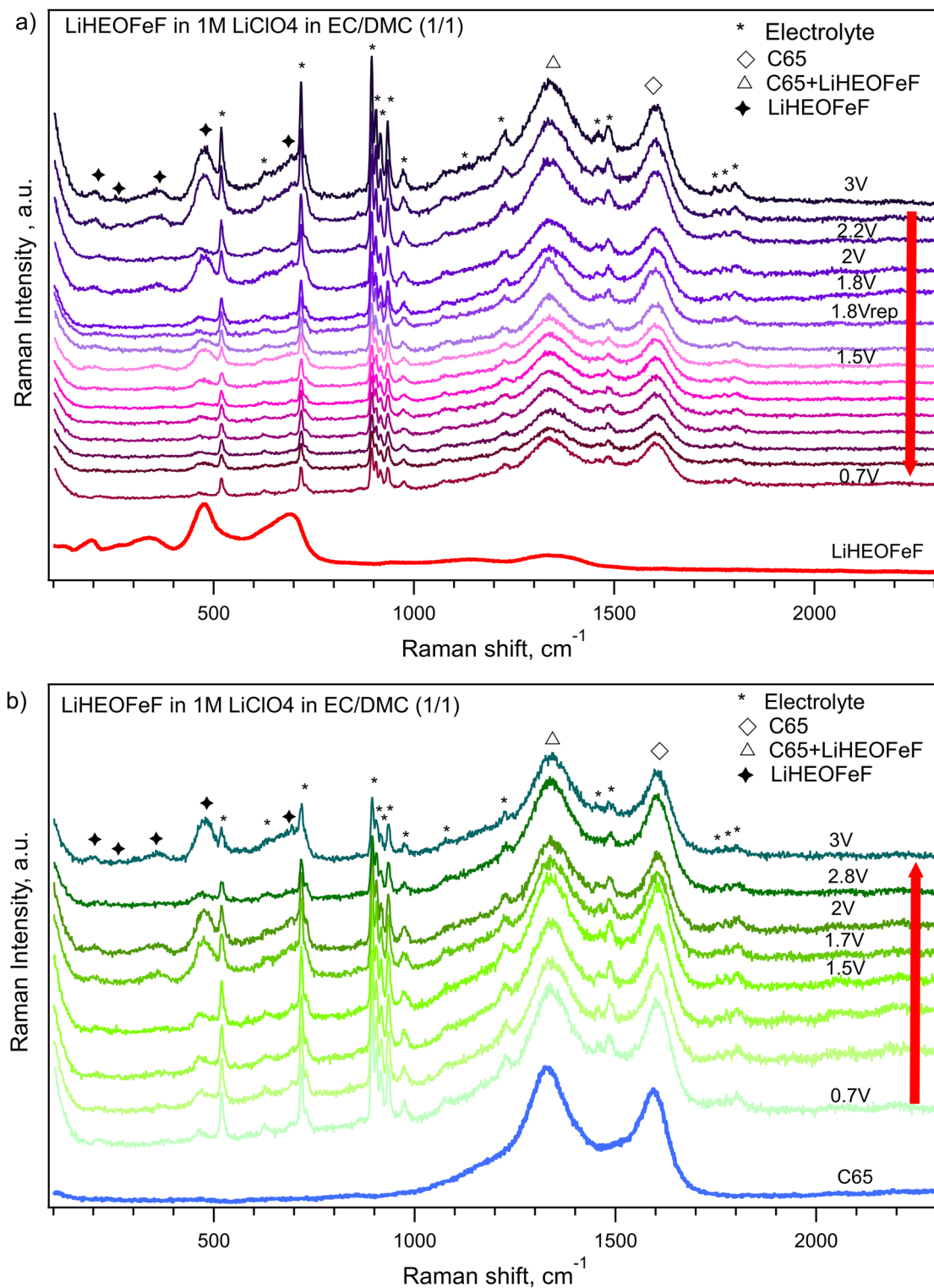
Fig. 8 In situ Raman spectroelectrochemical analysis of coin cells with the \text{LiHFeOFeF} cathode and 1\text{M LiClO}_4 in ethylene carbonate/dimethyl carbonate (1 : 1 by volume) as the electrolyte solution. (a) Charging of the coin cell from 3 V to 0.7 V vs. \text{Li}^+/\text{Li} . The Raman spectrum of blank \text{LiHFeOFeF} is also shown (red line). The label rep stands for repeated measurement at 1.8 V. (b) Discharging of coin cells from 0.7 V to 3 V vs. \text{Li}^+/\text{Li} . The Raman spectrum of the blank C65 additive is also shown (blue line). Spectra are offset, but the intensity scale is identical for all plots.
