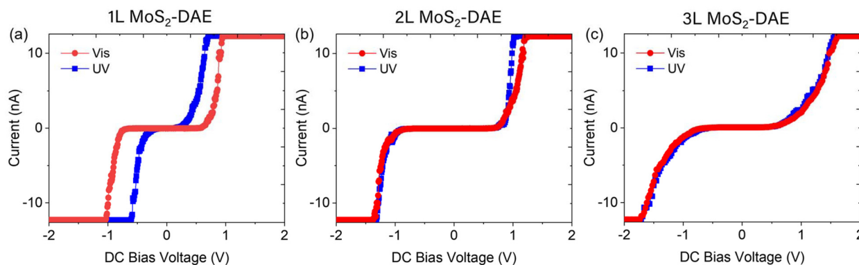
Fig. 3 Conductive AFM measurements on photoswitched hybrid samples under UV and visible irradiation: (a) 1L MoS 2 -DAE, (b) 2L MoS 2 -DAE, and (c) 3L MoS 2 -DAE. Bias DC voltage was applied from -2 V to 2 V and currents were recorded within \pm 12 nA. UV light enhances the current significantly in 1L MoS 2 -DAE, whereas no significant changes are observed from the hybrids with 2L and 3L MoS 2 .
