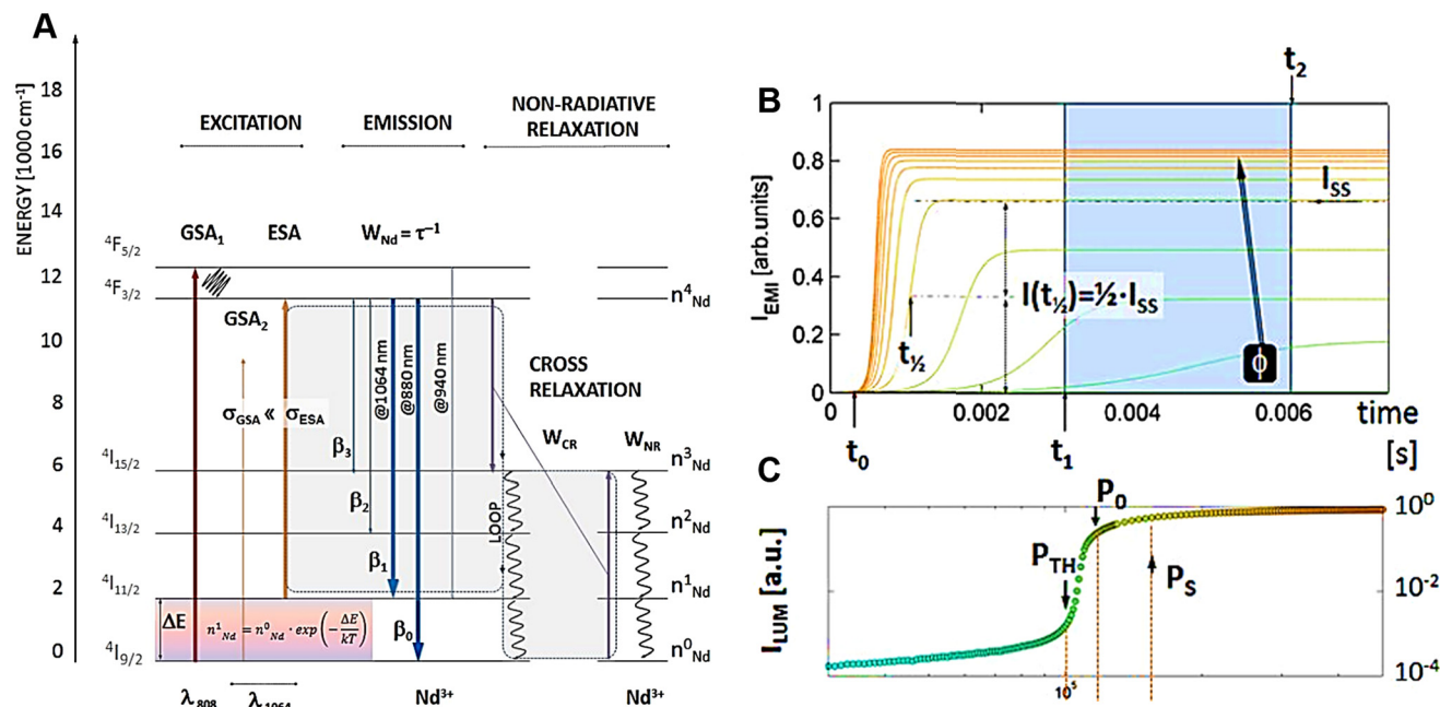
Fig. 4 PA in \text{Nd}^{3+} -doped nanoparticles. (A) Energy-level diagram of \text{Nd}^{3+} ions showing under 1064 nm photoexcitation resonant with ESA, radiative emission ( W_{\text{Nd}} ) from ^4\text{F}_{3/2} state and CR ( W_{\text{CR}} ) leading repeated population of the ^4\text{I}_{11/2} state. (B) The power-dependent PA emission profiles, ranging from green to orange, were simulated using a rate equation model for \text{Nd}^{3+} ions. Key parameters like steady-state intensity ( I_{\text{ss}} ), half-rise time ( t_{1/2} ), and time points ( t_0 , t_1 , t_2 ) were used to quantify the PA behavior. (C) The steady-state PA emission ( I_{\text{ss}} = I_{\text{LUM}}(t \rightarrow \infty) ). I_{\text{LUM}} represents luminescence intensity. Reproduced with permission from ref. 26. Copyright 2019, The Royal Society of Chemistry.
