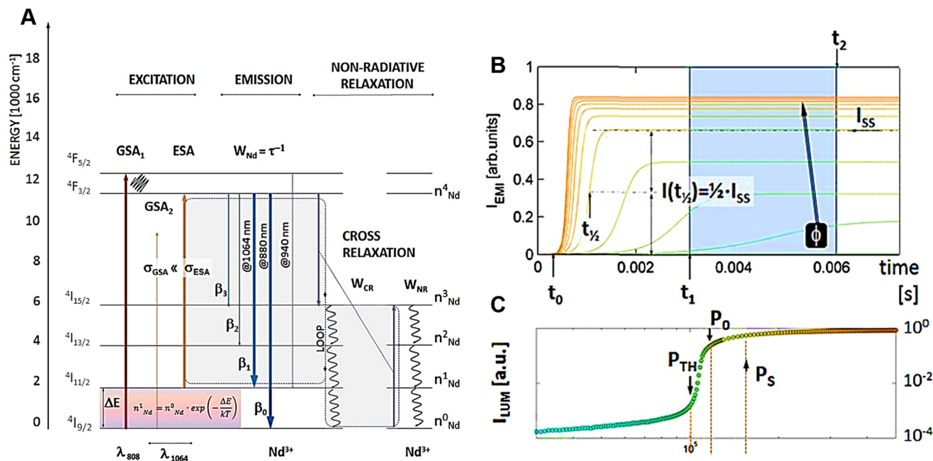
Fig. 4 PA in Nd 3+ -doped nanoparticles. (A) Energy-level diagram of Nd 3+ ions showing under 1064 nm photoexcitation resonant with ESA, radiative emission ( W_{Nd} ) from 4 F 3/2 state and CR ( W_{CR} ) leading repeated population of the 4 I 11/2 state. (B) The power-dependent PA emission profiles, ranging from green to orange, were simulated using a rate equation model for Nd 3+ ions. Key parameters like steady-state intensity ( I_{ss} ), half-rise time ( t_{1/2} ), and time points ( t_0 , t_1 , t_2 ) were used to quantify the PA behavior. (C) The steady-state PA emission ( I_{ss} = I_{LUM}(t \rightarrow \infty) ). I_{LUM} represents luminescence intensity. Reproduced with permission from ref. 26. Copyright 2019, The Royal Society of Chemistry.
