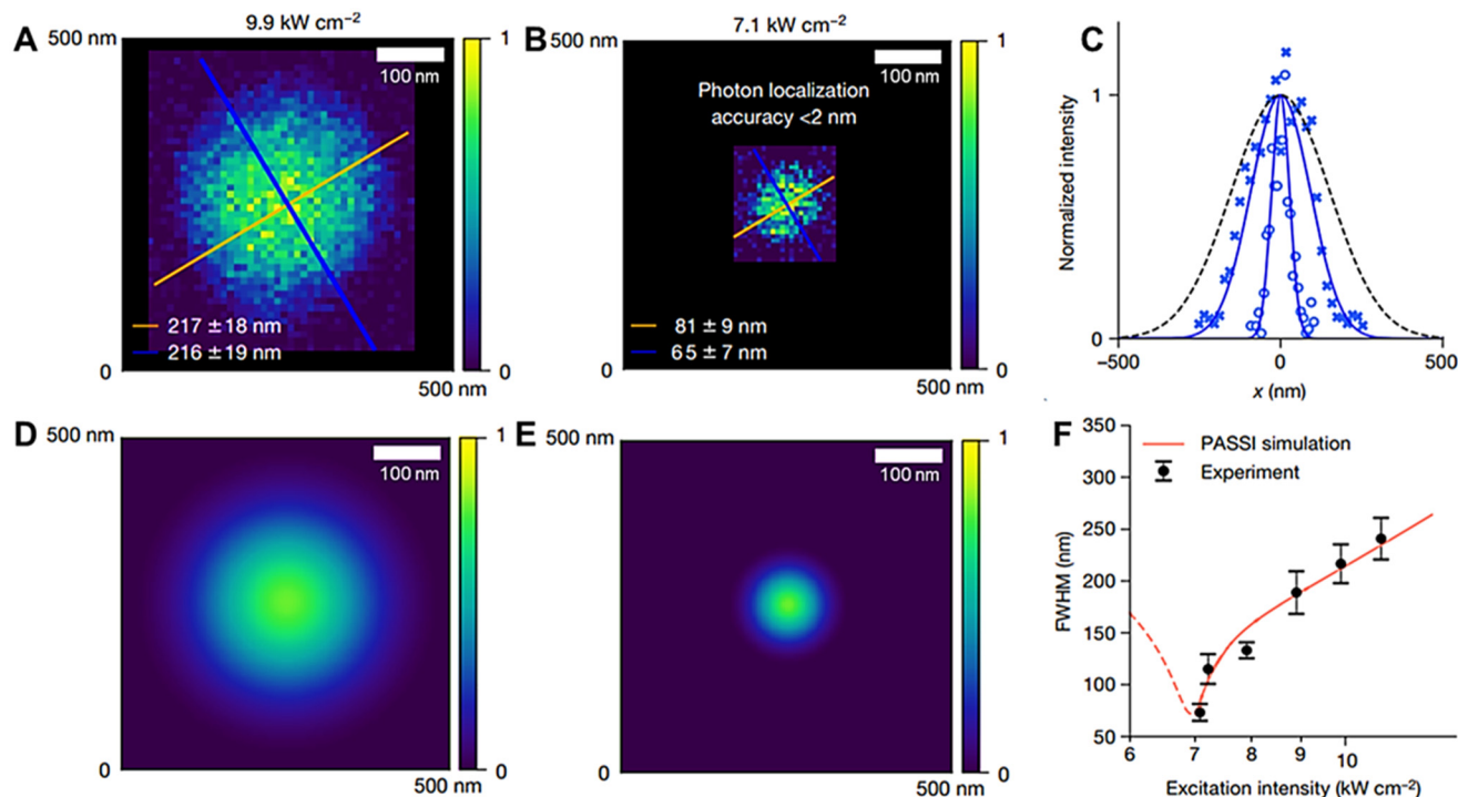
Fig. 10 Photon-avalanche single-beam super-resolution imaging. (A) Single-NP images excited under 1064 nm pump intensity at 9.9 \text{ kW cm}^{-2} (B) at 7.1 \text{ kW cm}^{-2} . (C) Line cuts corresponding to the blue lines in panels (A) and (B), along with a line cut through a theoretically diffraction-limited Gaussian focal spot. (D and E) ANP images are based on theoretical modeling under the same excitation wavelength and power intensities. (F) Comparison of measured (black) and simulated (red) FWHMs of single-NP PASSI images across different excitation intensities. Reproduced with permission from ref. 2. Copyright 2021, Springer Nature.
