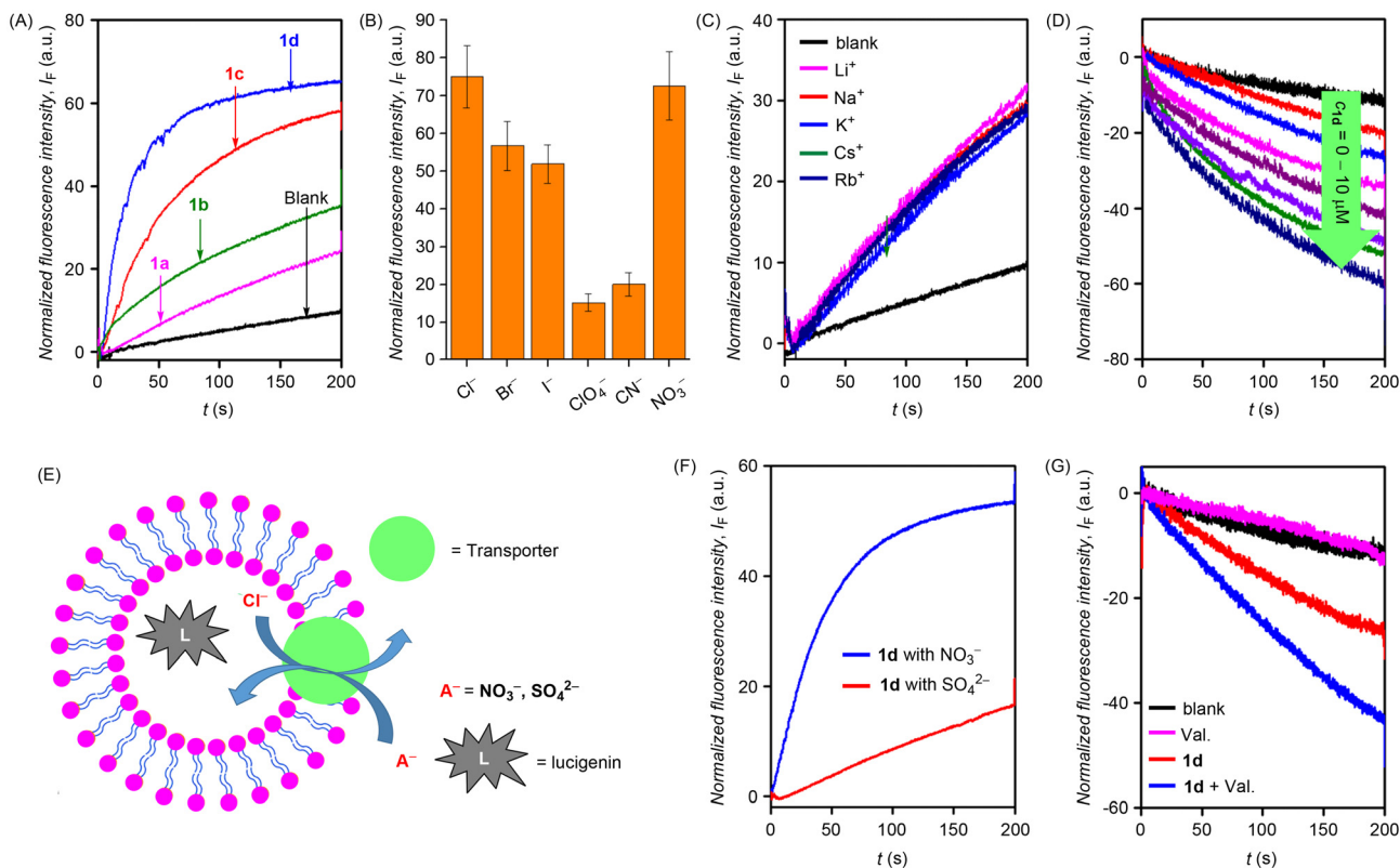
Fig. 2 Activity comparison of 1a–1d across EYPC-LUVs \supset HPTS (10.0 \mu\text{M} ) (A). Transport activity of 1d (5.0 \mu\text{M} ) by varying external anions across EYPC-LUVs \supset HPTS; each bar graph represents mean ion transport activity, calculated from three independent experiments (B). Transport activity of 1d (0.3 \mu\text{M} ) measured by varying external cations ( \text{M}^+ = \text{Li}^+, \text{Na}^+, \text{K}^+, \text{Rb}^+, \text{Cs}^+ ) across EYPC-LUVs \supset HPTS (C). Concentration-dependent activity of compound 1d across EYPC-LUVs \supset Lucigenin (D). Schematic representation of lucigenin-encapsulated antiport assay (E). Efflux of the \text{Cl}^- ion by 1d (10.0 \mu\text{M} ) in the presence of extravesicular \text{SO}_4^{2-} or extravesicular \text{NO}_3^- ions (F). Normalized \text{Cl}^- influx by 1d in the presence and absence of valinomycin (G).
