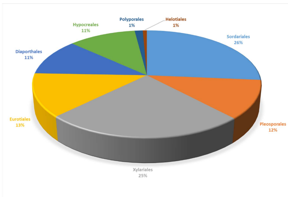
Fig. 48 Contribution of cytochalasins by different fungal orders.
