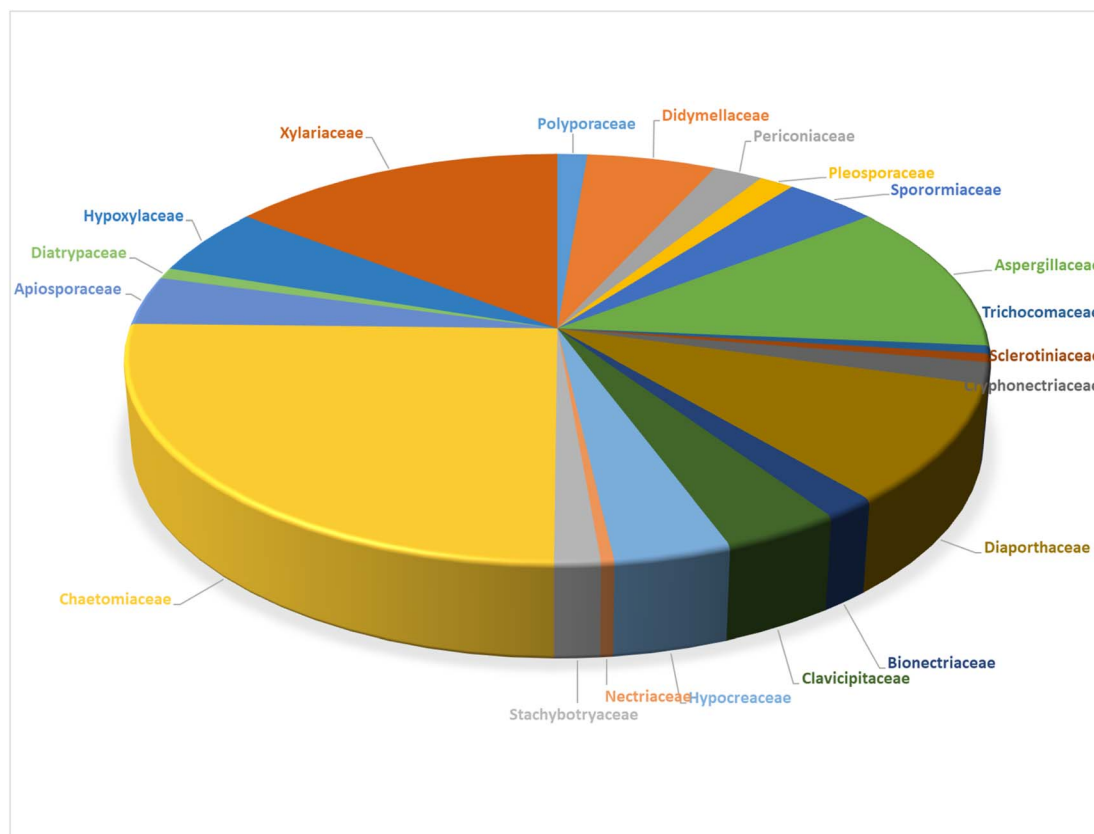
Fig. 49 Contribution of cytochalasins by various fungal families.
