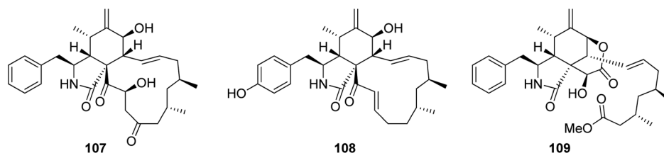
Fig. 13 Chemical structures of 107–109.
