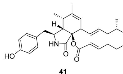
Fig. 5 Chemical structure of 41 .
