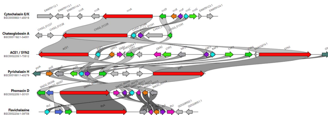
Chart 2 Chemical structures of biosynthetically investigated cytochalasans 192, 376, and I–VII.
