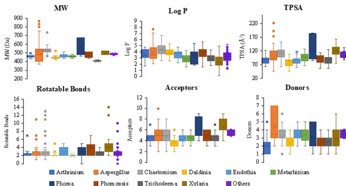
Fig. 43 Distribution of molecular weight (MW), octanol–water partition coefficient (log P ), number of rotatable bonds, topological polar surface area (TPSA), number of acceptors groups (acceptors), and number of donors groups (donors) by fungal genera, Arthrinium , Aspergillus , Chaetomium , Daldinia , Endothia , Metarhizium , Phoma , Phomopsis , Trichoderma , Xylaria , and Others.
