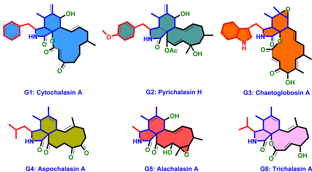
Chart 1 The molecular architecture of the six main cytochalasins (G1–G6).
