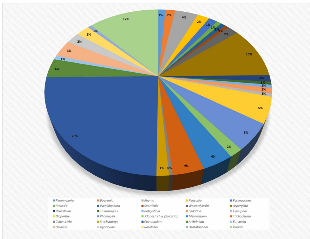
Fig. 50 Contribution of cytochalasans by different fungal genera.
