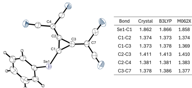
Fig. 2 Selected average bond lengths of 8 . Ellipsoids set at 50% probability. TDA cations omitted for clarity. Geometry optimization performed with B3LYP 20 and M06-2× 21 functionals, applying def2TZVP(D) 22 basis set.
