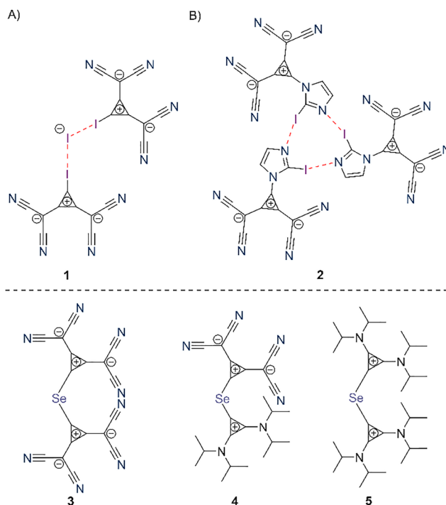
Fig. 1 Top: Previously reported cases of “anti-electrostatic” halogen bonded aggregates of 1,2-bis(dicyanomethylene)-cyclopropanide-containing synthons in the solid state: (A) – 2:1 anion binding and (B) – trimer formation. For (A): d_{I...N} = 85\% \Sigma r_{\omega} in (B): d_{I...N} = 79\text{--}81\% \Sigma r_{\omega} . Cations omitted for clarity. Bottom: Known cyclopropanide- and cyclopropanium-substituted chalcogen compounds. Counterions omitted for clarity.
