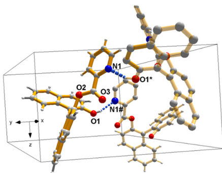
Fig. 1 View of the packing diagram of the benchmark L1 ligand showing the weak interaction ( D-H \cdots A/\tilde{A} : D \cdots A , H \cdots A ): O1-H1 \cdots N1^\# : 2.799(6), 1.985(5); \{\tilde{(\#)} 1 - y, x - y, 1/3 + z; (\ast) 1 - x + y, 1 - x, -1/3 + z\} .
