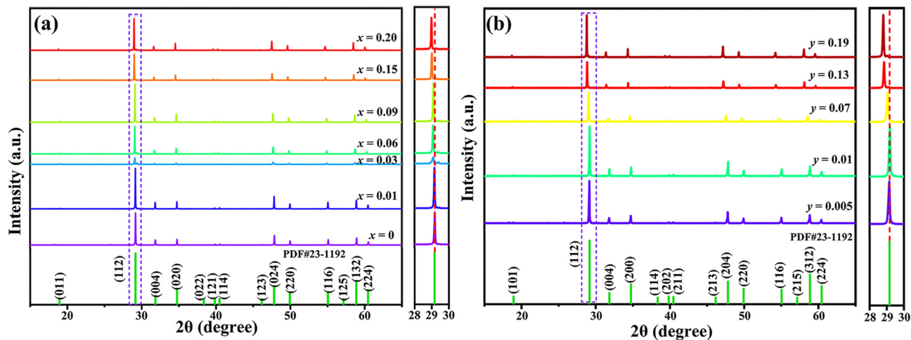
Fig. 1 PXRD patterns for (a) NLMO: x\text{Dy}^{3+} ( x = 0, 0.01, 0.03, 0.06, 0.09, 0.15, and 0.20 ) and (b) NLMO: 0.01\text{Dy}^{3+},y\text{Eu}^{3+} ( y = 0.005, 0.01, 0.07, 0.13, and 0.19 ) phosphors.
