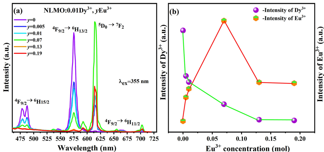
Fig. 6 (a) PL spectra of NLMO:0.01Dy 3+ , yEu 3+ ( y = 0.005, 0.01, 0.07, 0.13, and 0.19 ) phosphors; (b) line chart of emission intensity changes at 573 nm and 614 nm as the function of Eu 3+ concentration.
