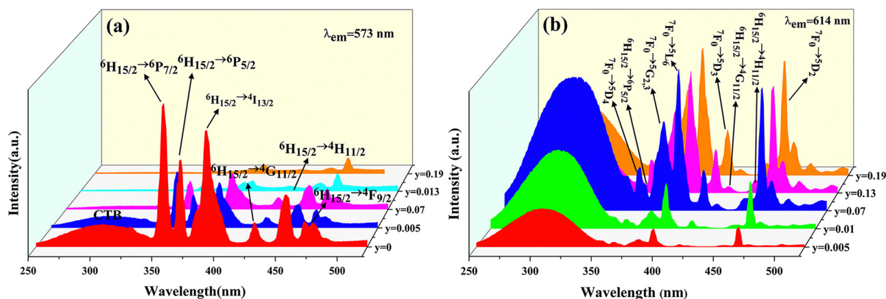
Fig. 5 PLE spectra of \text{NLMO}:0.01\text{Dy}^{3+},y\text{Eu}^{3+} ( y = 0.005, 0.01, 0.07, 0.13, \text{ and } 0.19 ) phosphors monitored at 573 and 614 nm, respectively.
