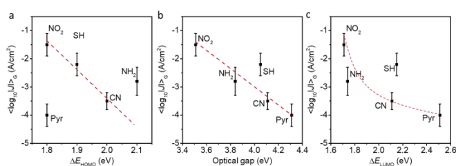
Figure 4. \langle \log_{10}|J| \rangle_G vs. \Delta E_{\text{HOMO}} (a), optical HOMO-LUMO gap (b), and \Delta E_{\text{LUMO}} (c) for Au-X(C 6 H 4 ) n H//GaO x /EGaIn junctions with X indicated in the plots. The error bars indicate \sigma_{\log,G} . The red dashed lines are visual guides.
