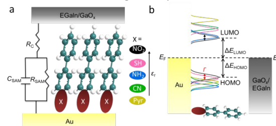
Figure 1. (a) Schematic illustration of the Au-X(C 6 H 4 ) n H//GaO x /EGaIn junction with n =1 or 2 and X=-NO 2 , -SH, -NH 2 , -CN, and -Pyr where “-” indicates covalent bond, “//” indicates the non-covalent contact and “/” represents the
