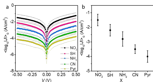
Figure 3. (a) Curves of \langle \log_{10}|J| \rangle_G vs. V of Au-X(C 6 H 4 ) n H//GaO x /EGaIn junctions. (b) \langle \log_{10}|J| \rangle_G vs. X for all the junctions. The dashed lines in Panel a and error bars in Panel b indicate the Gaussian logarithmic standard deviation, \sigma_{\log,G} .
