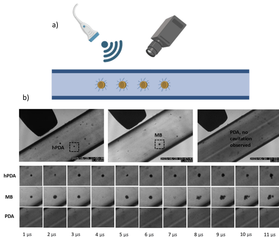
Fig. 6 Cavitation of different types of particles under ultrasound application. (a) Illustration of the experimental set-up; NPs are injected into a 500 μm polycarbonate capillary and exposed to 100 cycles at 1.1 MHz ultrasound. Cavitation events are captured using a high-speed camera. (b) Cavitation clouds captured over 11 μs for hollow polydopamine nanoparticles (hPDA) compared to commercially available microbubbles (MB) and polydopamine (PDA) controls.
