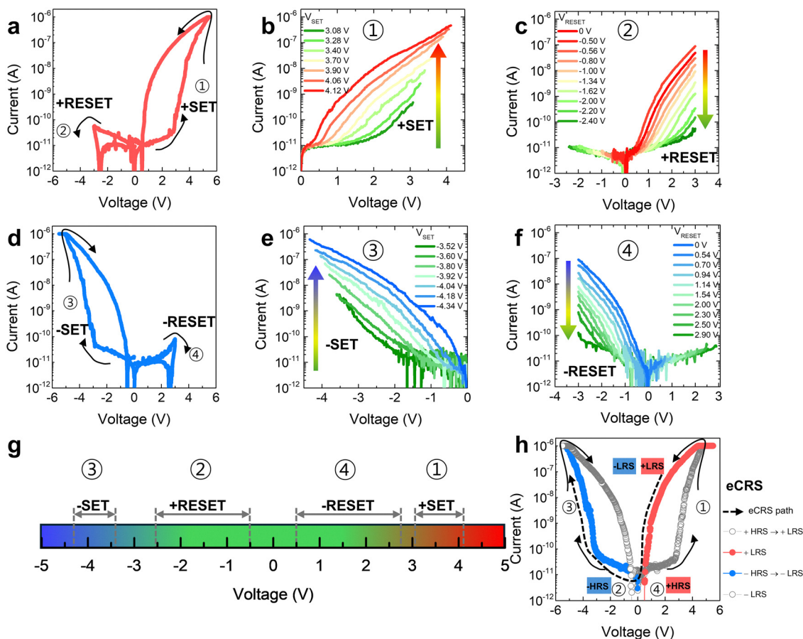
Fig. 2 (a) Positive eBRS operation of the THT device with a +SET voltage of 5 V, a compliance current of 1 \mu\text{A} and a +RESET voltage of -3 \text{ V} . (b) Gradual SET switching from +HRS to +LRS with different set sweep voltages (3.08 V to 4.12 V). (c) Rectifying RESET switching from +LRS to +HRS with different reset sweep voltages from -0.50 \text{ V} to -2.40 \text{ V} , confirmed by a 3.0 \text{ V} single sweep after each reset sweep. (d) Negative eBRS operation of the THT device. (e) Gradual -SET switching from -HRS to -LRS with different set sweep voltages ( -3.52 \text{ V} to -4.34 \text{ V} ). (f) Rectifying -RESET switching from -LRS to -HRS with different reset sweep voltages (from 0.54 \text{ V} to 2.90 \text{ V} ) confirmed by a -3.0 \text{ V} single sweep after each reset sweep. (g) A schematic diagram showing the THT device operation voltages with positive eBRS and negative eBRS. (h) eCRS with BSR operation obtained by the consecutive operation of positive eBRS and negative eBRS: switching from +HRS to +LRS, then resetting to -HRS , and back to -LRS .
