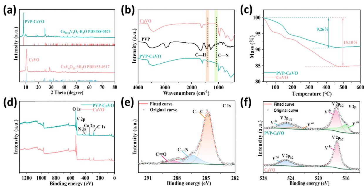
Fig. 2 (a) XRD patterns of CaVO and PVP-CaVO. (b) FT-IR plots of CaVO and PVP-CaVO. (c) TGA curves of CaVO and PVP-CaVO. (d) The full XPS survey spectra of CaVO and PVP-CaVO. (e) C 1s XPS spectra of PVP-CaVO. (f) V 2p XPS spectra of CaVO and PVP-CaVO.
