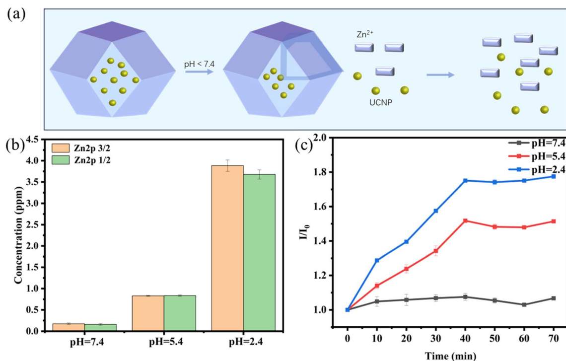
Fig. 5 (a) Schematic diagram of UCNPs@ZIF-8 cracking under acidic conditions; (b) \text{Zn}^{2+} concentration in different pH solutions; (c) recovery of the luminescence intensity of the UCNP under different pH environments.
