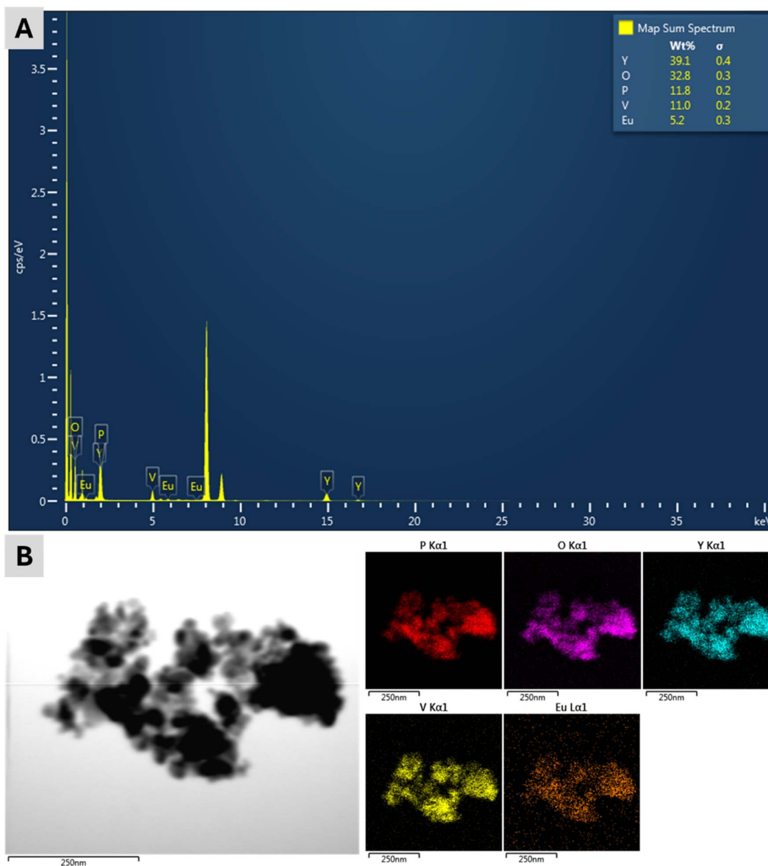
Fig. 4 (A) EDX spectra and (B) mapping of elements in the Y(P_{0.5}V_{0.5})O_4:5\% Eu sample.
