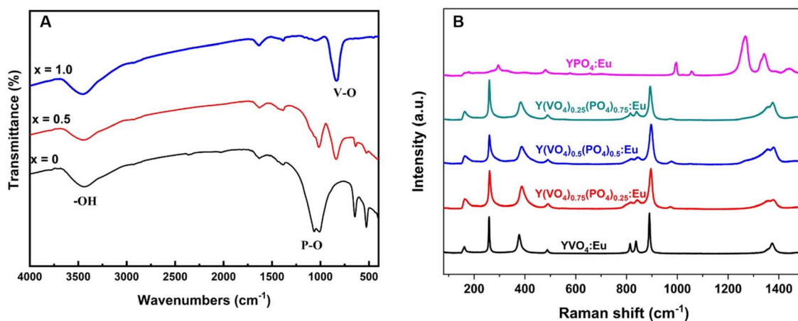
Fig. 2 (A) FTIR and (B) Raman spectra of YP_{(1-x)}V_xO_4:5\% Eu materials.
