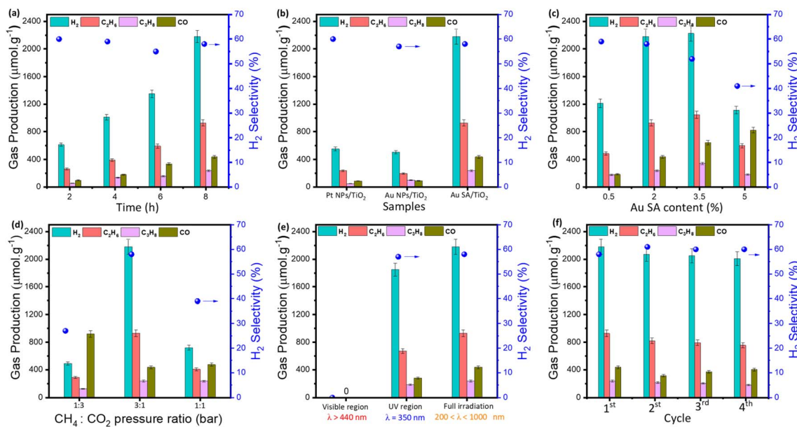
Fig. 7 Photocatalytic methane oxidation performances and the H 2 selectivity as a function of reaction time over the standard Au SA/TiO 2 sample (2 wt% Au) (a), comparable photocatalytic experiments of different catalysts (b), comparison of photocatalytic activity with different Au loading contents, reactant ratios, and irradiation regions, respectively (c)–(e), and stability tests over four cycles (f). Reaction conditions: 50 mg of the standard Au SA/TiO 2 catalyst with 2% Au loading, CH 4 : CO 2 = 3 : 1 (stand pressure ratio), xenon lamp 300 W. In figures (a), (d) and (f), standard Au SA/TiO 2 was used.
