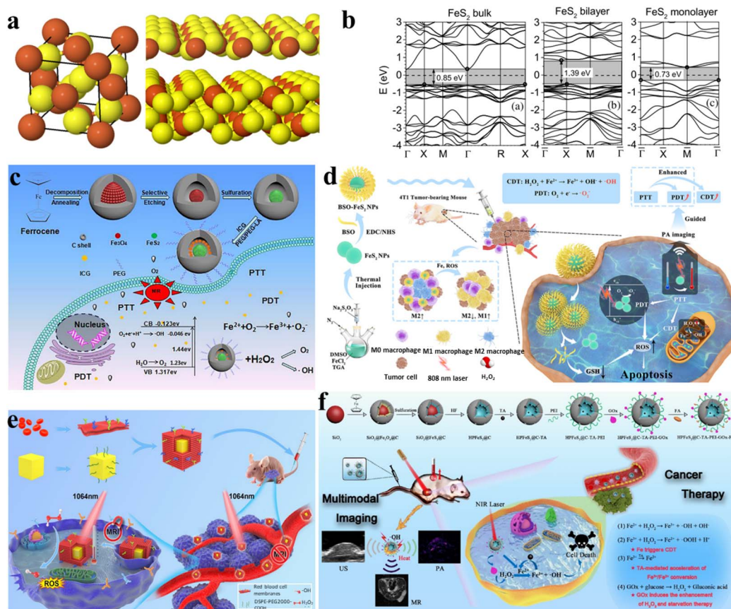
Fig. 5 (a) Models of \text{FeS}_2 in bulk, monolayer, and bilayer forms, with S atoms in yellow and Fe atoms shown in brown. 84 (b) Band structures and densities of states (DOS) for bulk, bilayer, and monolayer \text{FeS}_2 , with shaded regions indicating the band gaps. 84 (c) Combining PTT, PDT, and multimode imaging into a single nanoplatform. 86 (d) Illustration of PAI-guided PTT, CDT and PDT mediated by BSO- \text{FeS}_2 . 87 (e) Schematic depicting the in vivo fabrication and anti-tumor impact of \text{FeS}_2 @RBCs. The RBC coating results in extended blood circulation, enhancing tumor accumulation. 88 (f) Preparation procedure and therapeutic mechanism of HP \text{FeS}_2 @C-TA-PEI-GOx-FA. 89
