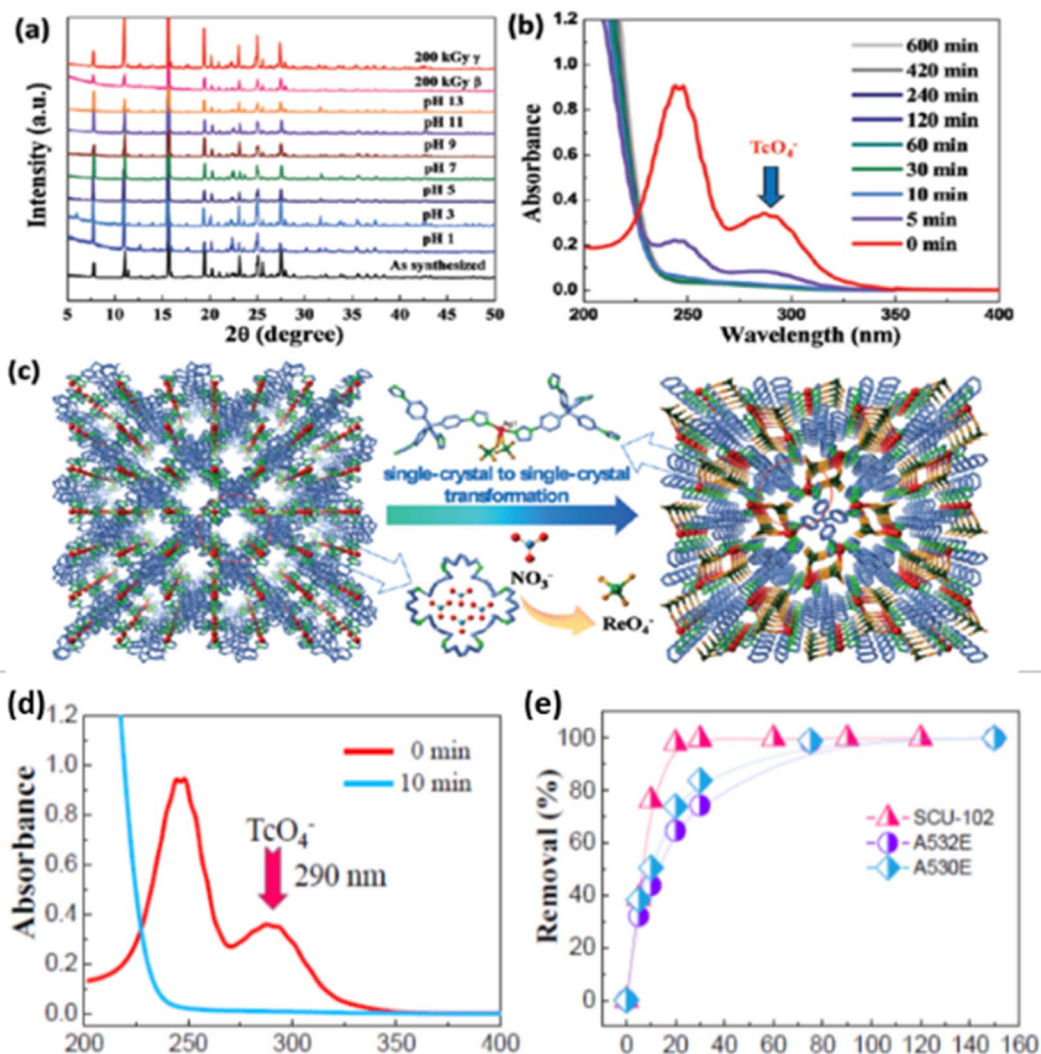
Fig. 4 (a) The stability of the SCU-100 MOF with respect to different pH and radiation. (b) Its sorption properties with respect to TcO 4 - as a function of contact time. (c) The transformation of a single crystal into another single crystal throughout the sorption process. Reproduced from ref. 37 with permission from American Chemical Society. (d) UV-vis spectra of 99 TcO 4 - ions during the anion exchange with the SCU-102 MOF, plotted against contact time. (e) A comparison of the ReO 4 - sorption kinetics by Purolite A532E, SCU-102, and A530E resins. Reproduced with permission from ref. 51.
